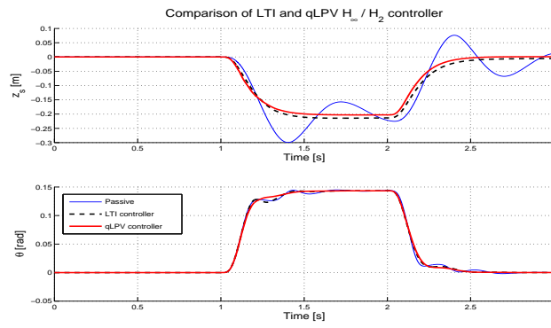
Figure 6: Comparison of LTI (dashed) and qLPV (solid) mixed synthesis performances
