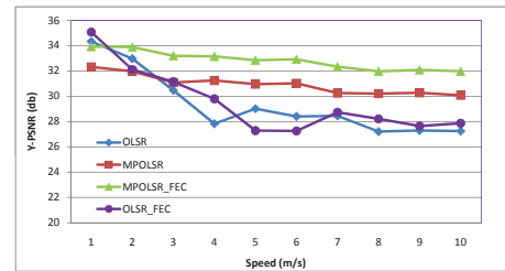
Fig. 5. The quality of video transmission through the different protocols (with or without FEC code)
