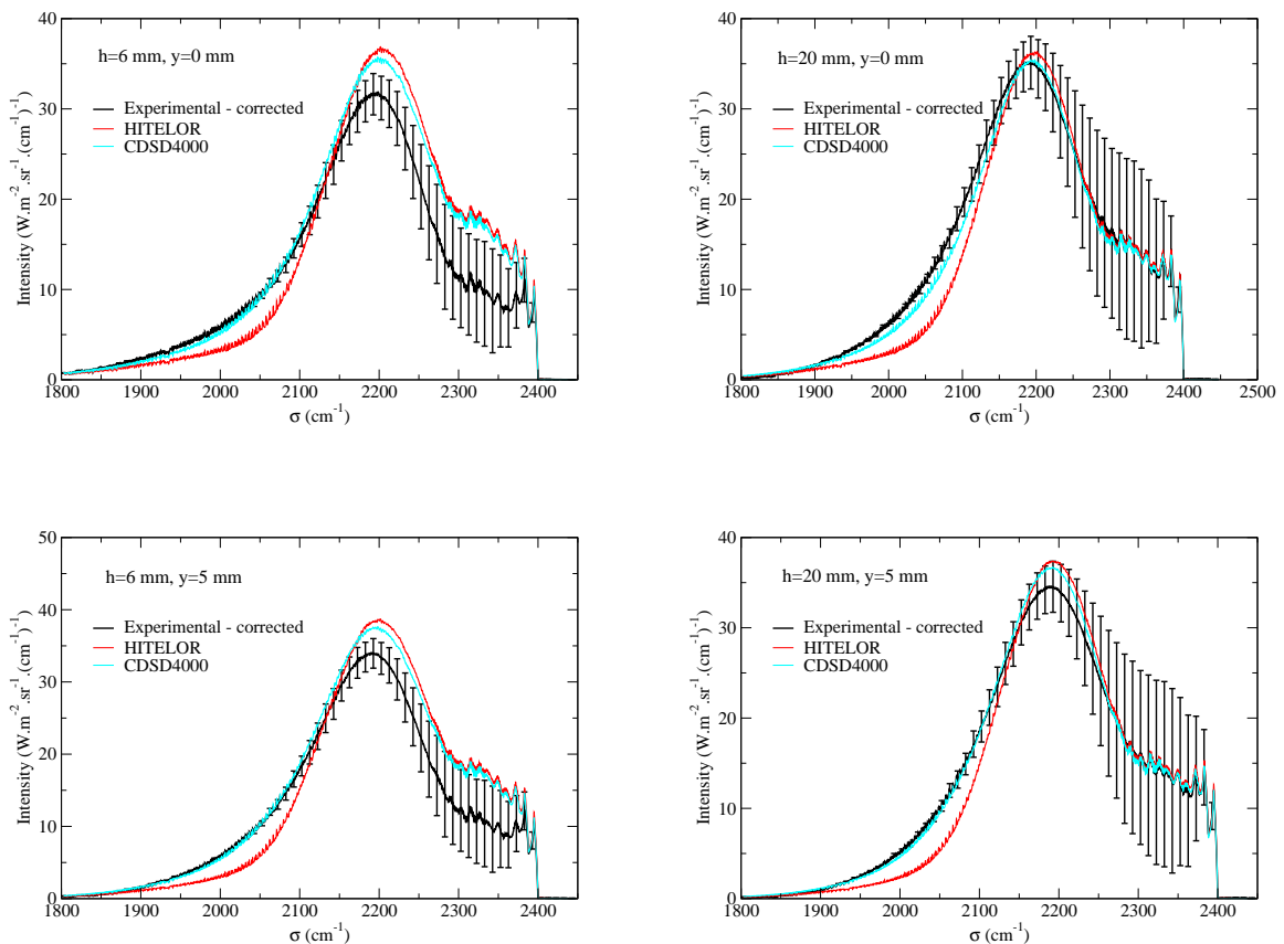
Figure 5: Experimental (corrected) and theoretical line of sight integrated intensities at h=6 mm (left) and h=20 mm (right) and for y=0 (central chord) and y=5 mm ; sapphire tube ; 4.3 \mu\text{m} region.
