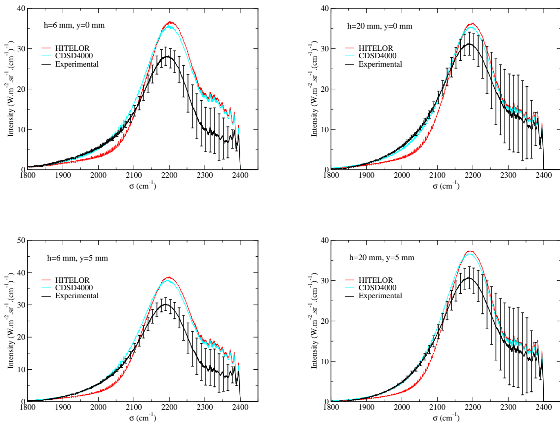
Figure 4: Experimental and theoretical line of sight integrated intensities at h=6 mm (left) and h=20 mm (right) and for y=0 (central chord) and y=5 mm ; sapphire tube ; 4.3 \mu\text{m} region.
