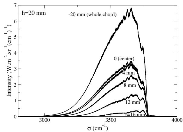
Figure 6: Partial intensities on the central chord computed with CDSD-4000 and the temperature profile obtained with a sapphire tube at h=6 mm and h=20 mm.
