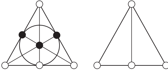
Figure 3: An illustration of a hypothetical case where three of the four observables would lie on a line of the Fano plane.
