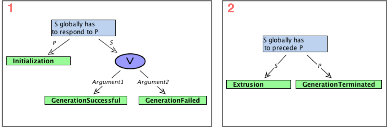
Fig. 7. Two constraints from the category actionOrder : (1) "After it is initialized, the generator either finishes successfully or fails.", (2) "The extrusion phase has to be executed before the generation terminates."
