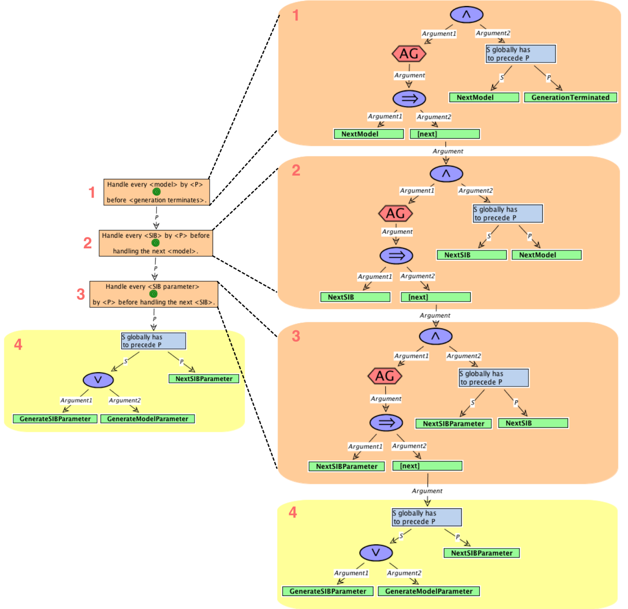
Fig. 9. A constraint checking for the complete handling of input SLGs, using the new “Handle By” pattern
