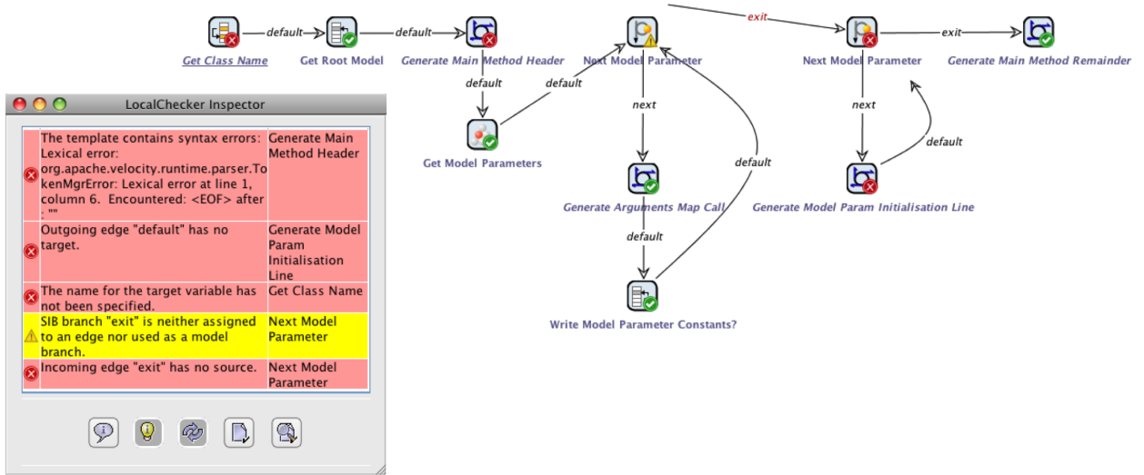
Fig. 4. Checking local constraints with the LocalChecker
