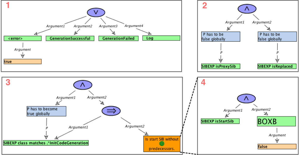
Fig. 6. Three constraints from the category actionOccurrence : (1) "All errors are handled or at least logged, otherwise the generation fails or finishes successfully.", (2) "No proxy SIBs.", (3) & (4) SIB InitCodeGeneration is used and is a start SIB without any predecessors.
