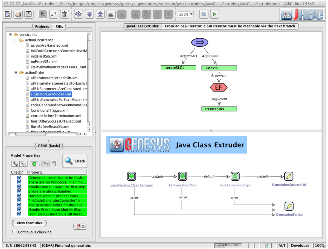
Fig. 5. Verifying the Java Class Extruder with GEAR & the FormulaBuilder
