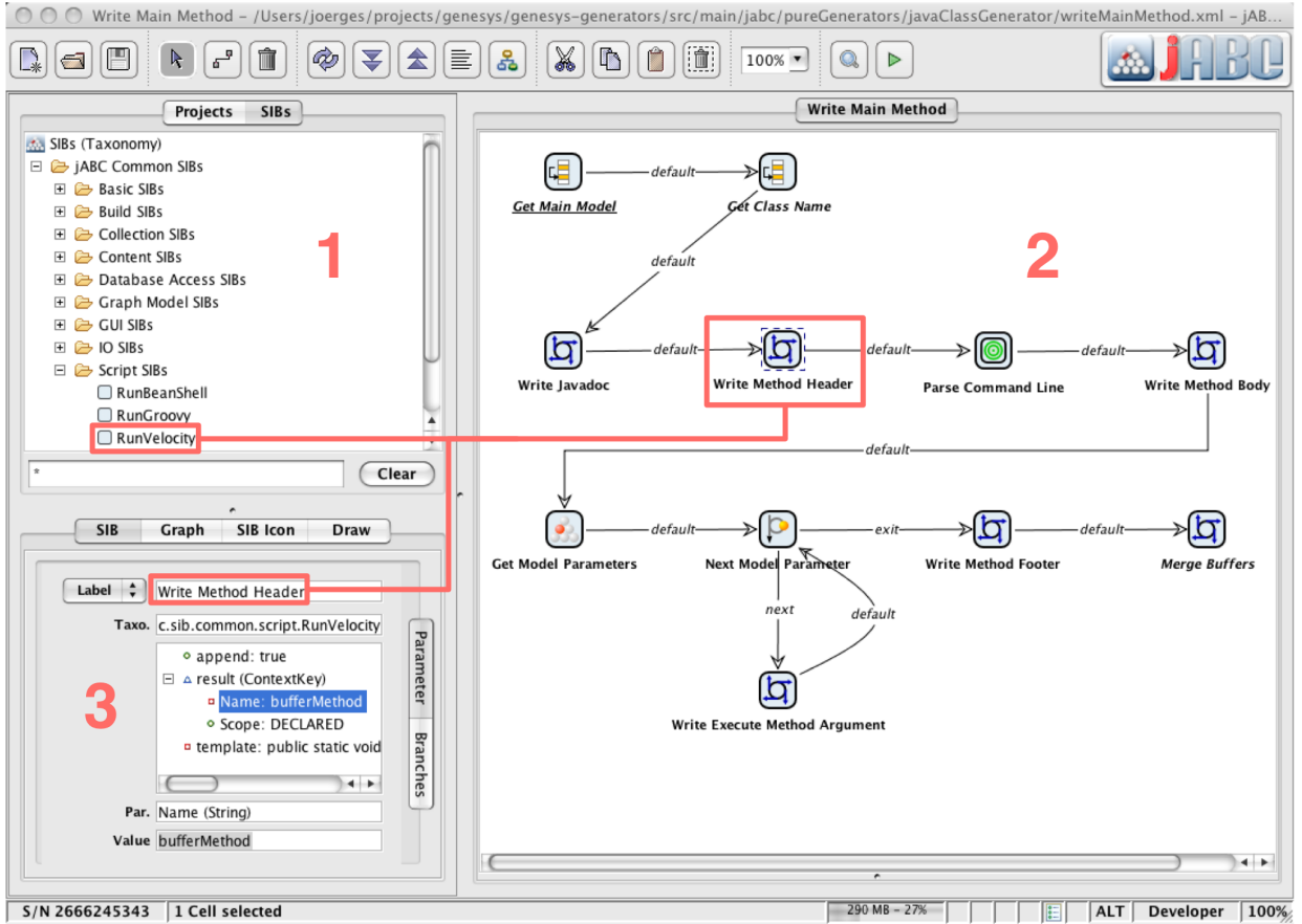
Fig. 2. The user interface of jABC
