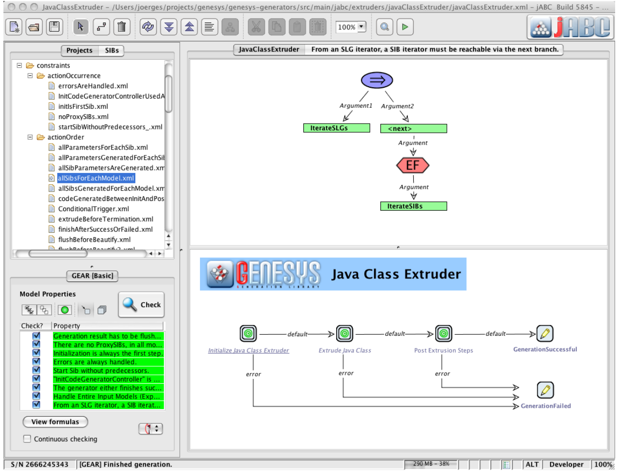
Fig. 5. Verifying the Java Class Extruder with GEAR & the FormulaBuilder
