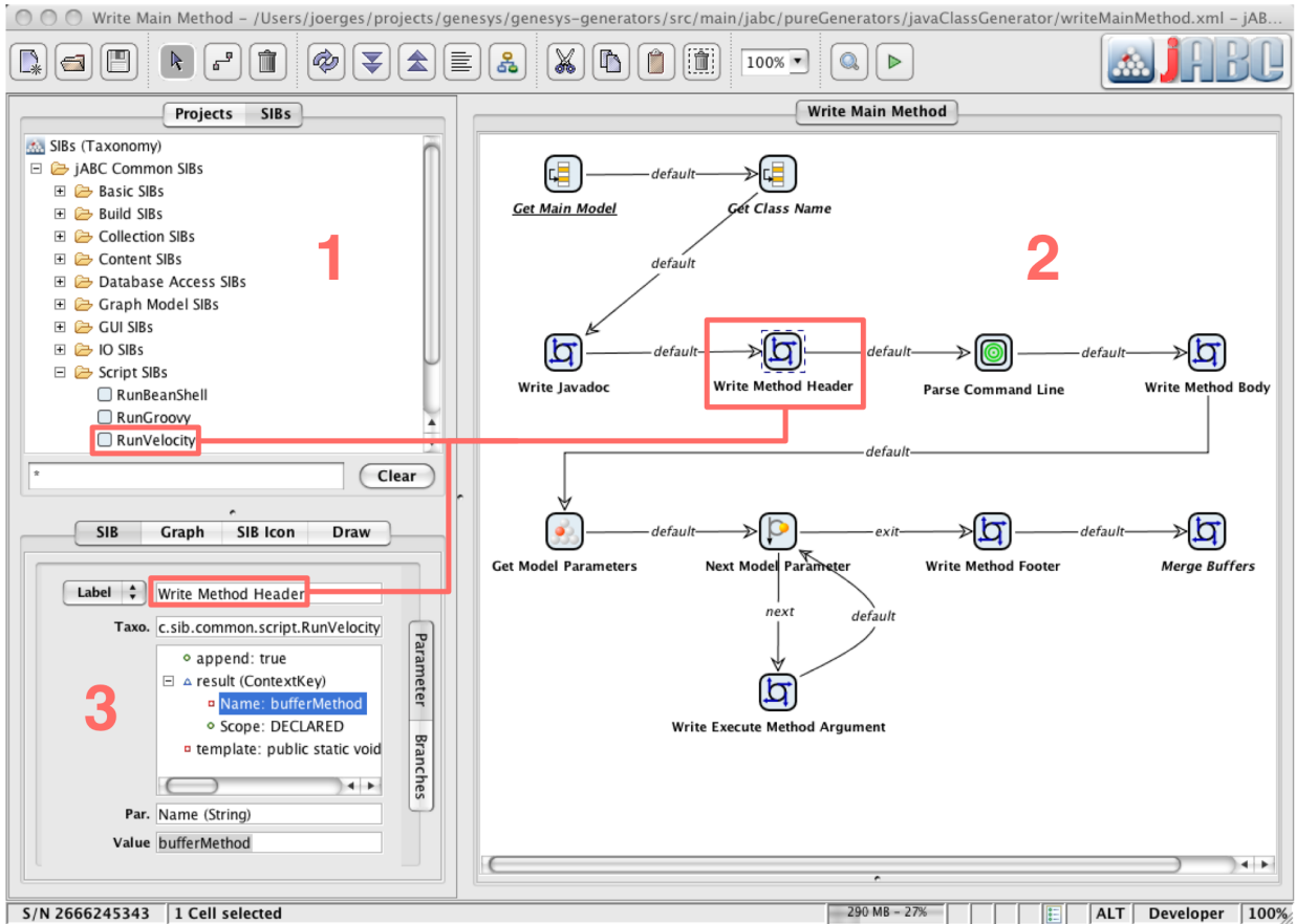
Fig. 2. The user interface of jABC
