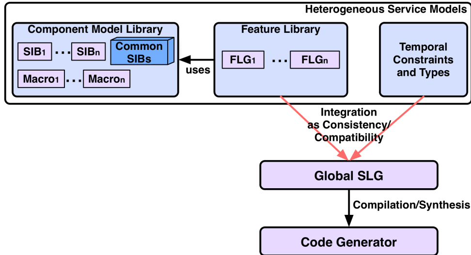
Fig. 1. XMDD with jABC & Genesys
