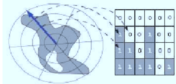
Figure 20: Shape matrix.
