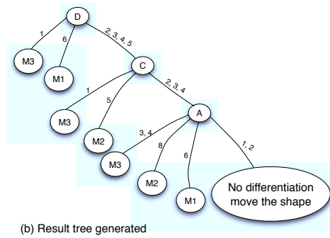
Figure 8: An example of the result tree of criteria values according to a combination of criteria and a set of models.
