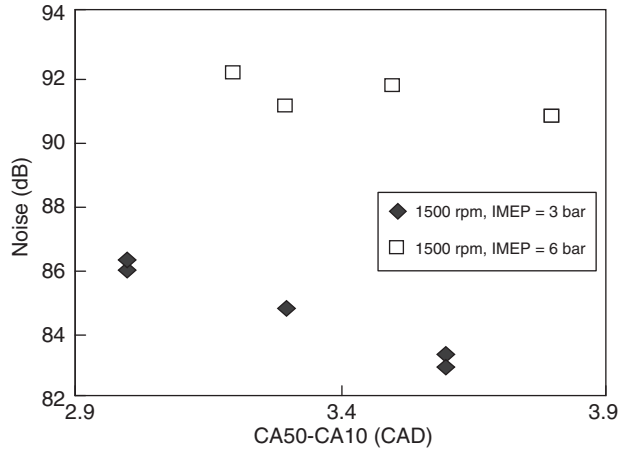
Figure 6 Noise versus combustion propagation time between the CA10 and the CA50.
