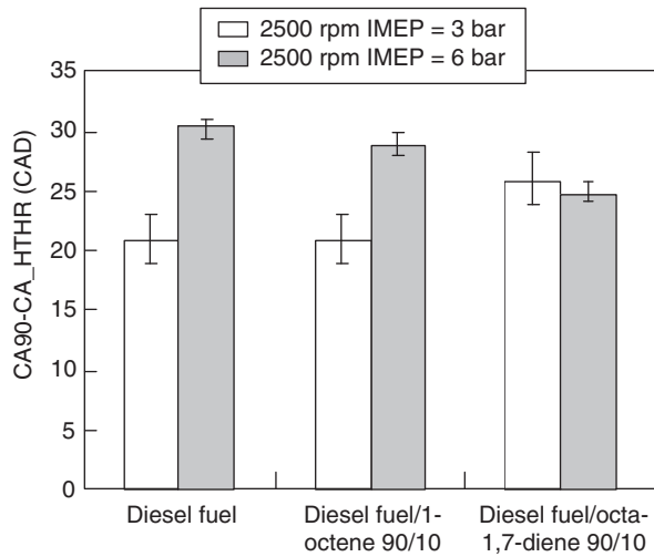
Figure 16 Olefin effect on the time of the end of the combustion between the peak of the HTHR and the CA90 of the Diesel base fuel at 2500 rpm.
