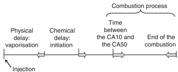
Figure 8 Schematic representation of the modifications needed to improve the HCCI combustion.
