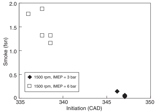
Figure 5 Smoke emissions versus initiation of the combustion.
