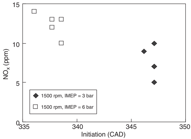
Figure 4 NO x emissions versus initiation of the combustion.
