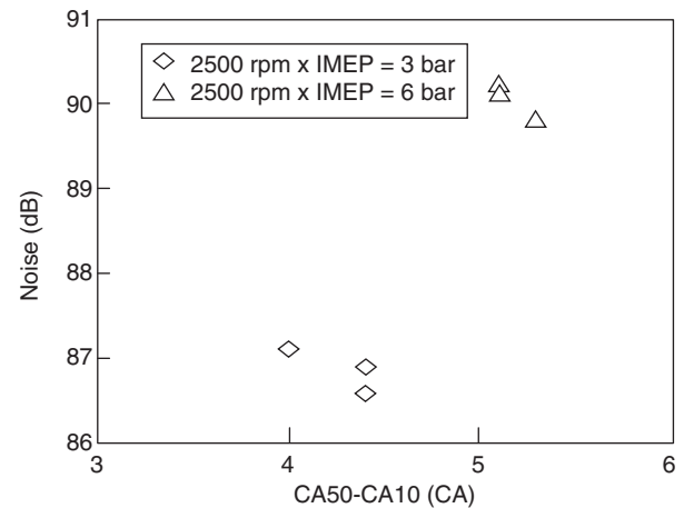
Figure 19 Noise versus CA50-CA10 at 2500 rpm.
