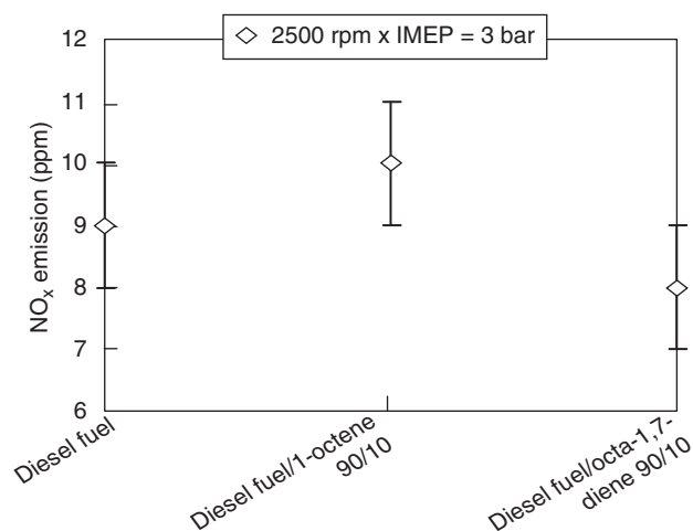
Figure 25 Olefin effect on NO x emissions at 2500 rpm × IMEP = 3 bar.
