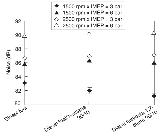
Figure 17 Olefin effect on the noise.
