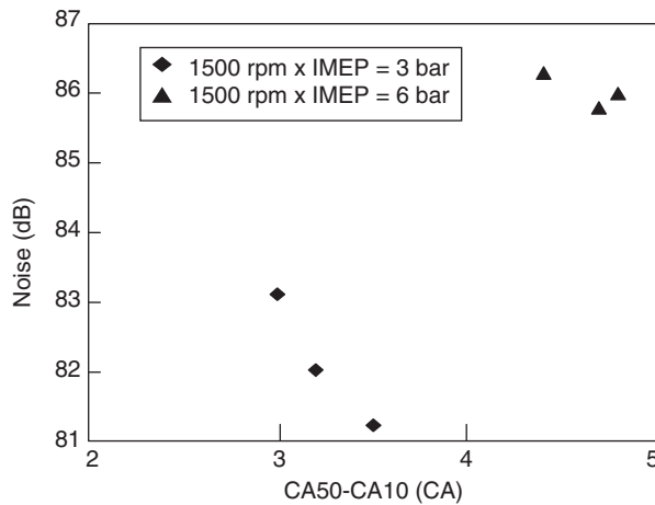
Figure 18 Noise versus CA50-CA10 at 1500 rpm.
