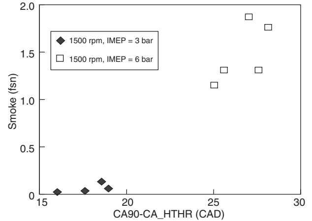
Figure 7 Smoke emissions versus time of the end of the combustion between the peak of the HTHR (CA_HTHR) and the CA90.
