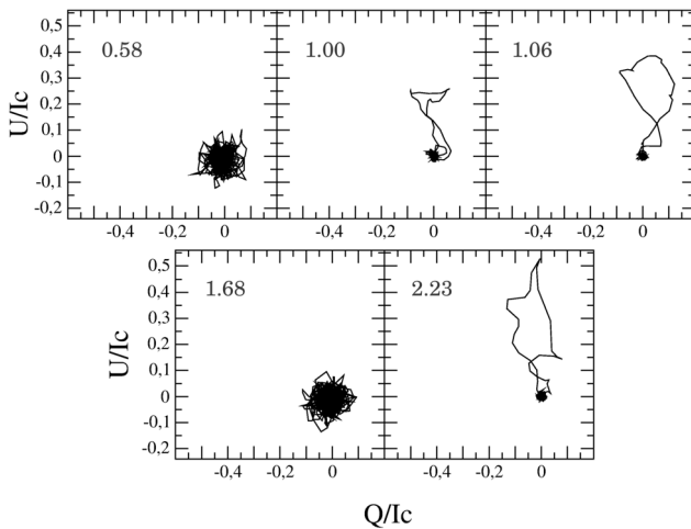
Fig. 9. Hydrogen Balmer lines signatures of cycles 1 and 2 of our monitoring of o Ceti in H \delta ( u(q) ). See Fig. 3.
