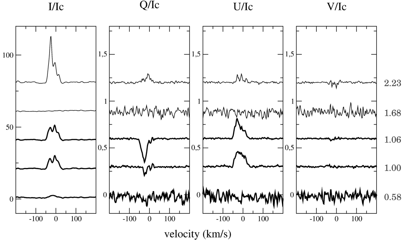
Fig. 6. Hydrogen Balmer line signatures of cycles 1 (thick lines) and 2 (thin lines) of our monitoring of o Ceti in Hy (full Stokes). See Fig. 2.
