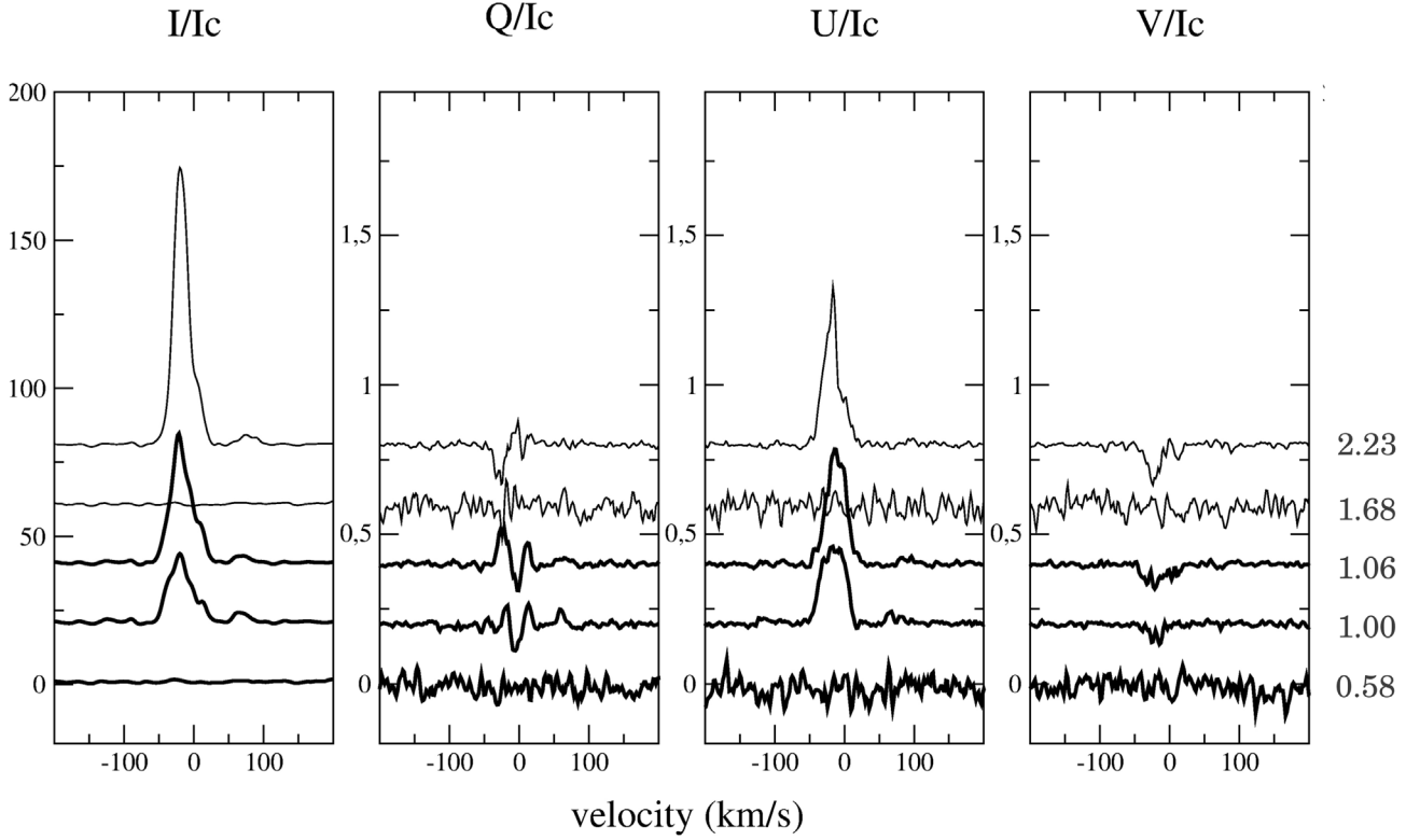
Fig. 8. Hydrogen Balmer line signatures of cycles 1 (thick lines) and 2 (thin lines) of our monitoring of o Ceti in H \delta (full Stokes). See Fig. 2.
