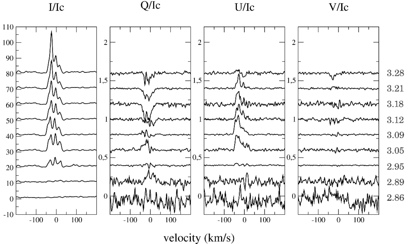
Fig. 2. Hydrogen Balmer line signatures of the third cycle of our monitoring of o Ceti in H \gamma (full Stokes). Successive signatures are artificially offset vertically for legibility. Phases are indicated on the right (see Table 1).
