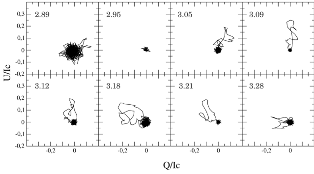
Fig. 3. Hydrogen Balmer line signatures of the third cycle of our monitoring of o Ceti in H\gamma ( u(q) ). Phases are indicated in the topleft of each frame (see Table 1).
