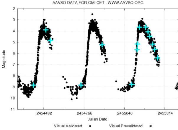
Fig. 1. Light curve of o Ceti (from AAVSO website) for the three cycles of the survey. Each blue cross is one spectropolarimetric observation of our survey.
