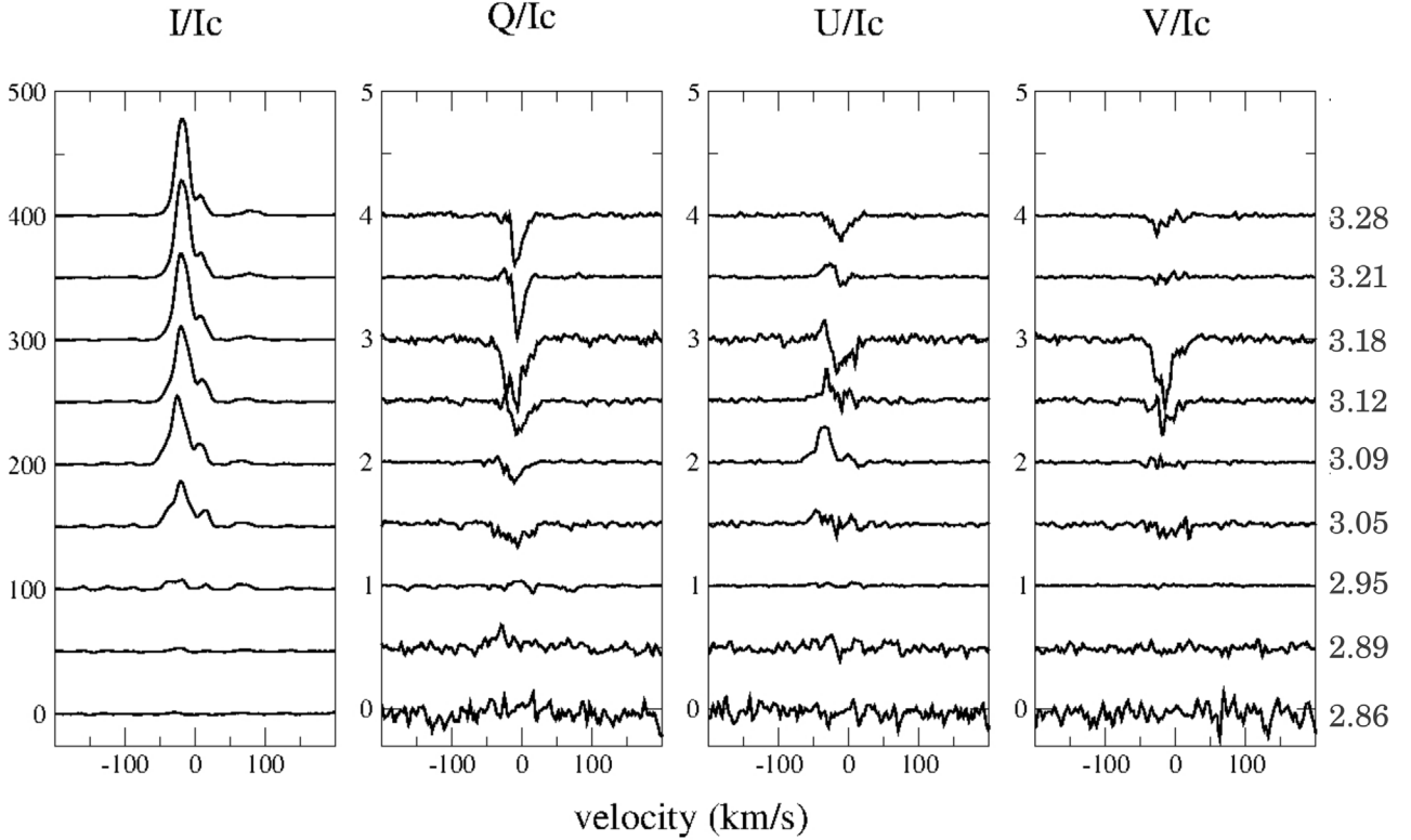
Fig. 4. Hydrogen Balmer line signatures of the third cycle of our monitoring of o Ceti in H\delta (full Stokes). See Fig. 2.
