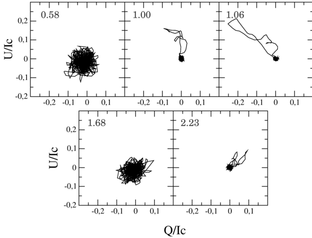
Fig. 7. Hydrogen Balmer line signatures of cycles 1 and 2 of our monitoring of o Ceti in Hy ( u(q) ). See Fig. 3.
