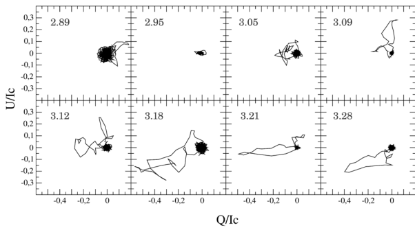
Fig. 5. Hydrogen Balmer line signatures of the third cycle of our monitoring of o Ceti in H\delta ( u(q) ). See Fig. 3.
