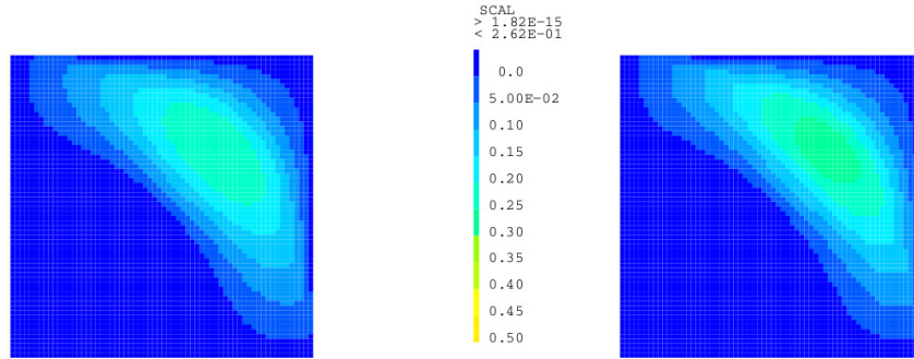
Figure 1: Concentration on a grid made of 4096 squares for the first correction (maximum value 0.26, minimum value 1.82 \times 10^{-15} ) and the regularized correction (maximum value 0.29, minimum value 7.95 \times 10^{-10} ).
