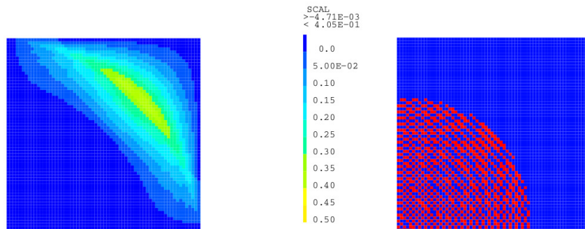
Figure 2: Concentration and position of the undershoots (in red) for the initial scheme on a grid made of 4096 cells (maximum value 0.41, minimum value -4.71 \times 10^{-3} ).
