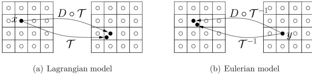
Figure 2: Image transformation models: (a) Lagrangian and (b) Eulerian. (a) and (b) left: image support before transformation, right: image support after transformation. The digital support S \subset \mathbb{Z}^2 is depicted by white dots. The Voronoi cells of E associated to the points of S are depicted by squares.
