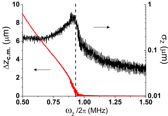
FIG. 4. (color online) Relative distance between the c.m. of the two rings, \Delta z_{\text{c.m.}} (red curve, left axis), and standard deviation of the axial component of the ion's positions from the c.m. position of the ring of which they belong, \sigma_z (black curve, right axis), function of the increasing axial confinement frequency \omega_z . The vertical dashed line marks the theoretical transition from the double-ring to single-ring configuration.
