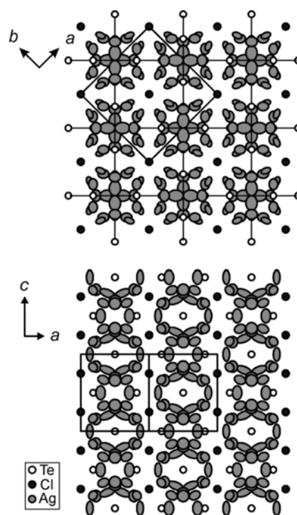
Fig. 2. Crystal structure sections of \alpha\text{-Ag}_5\text{Te}_2\text{Cl} (573 K). The silver ions are forming a strand of delocalized silver along the c axis. Displacement parameters are shown at the 50% level.
