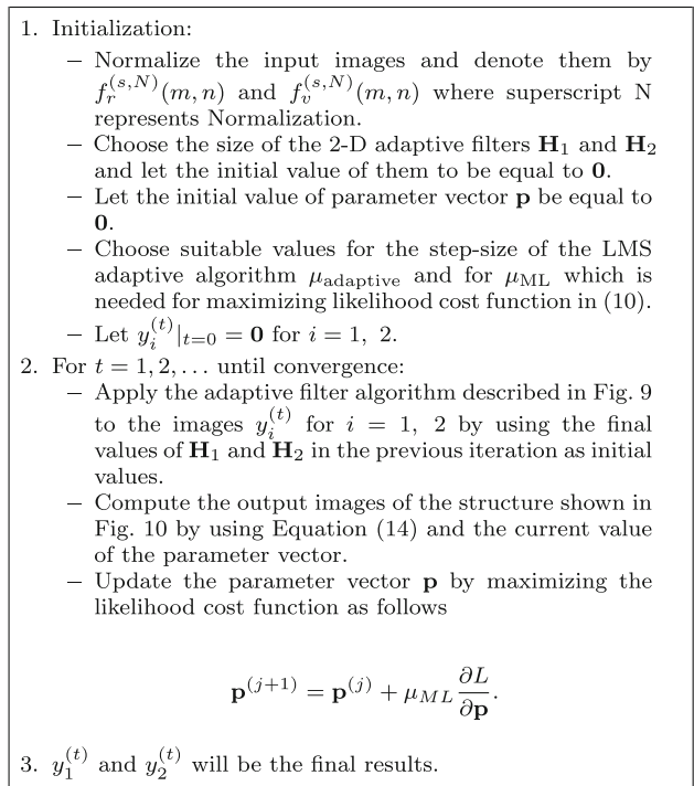
Fig. 11 Proposed algorithm for removing show-through and blurring effect
