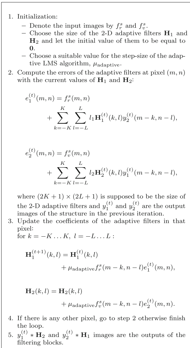
Fig. 9 Algorithm for estimating the adaptive filters of Fig. 8
