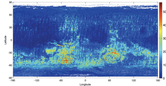
Figure 10: The extended rock abundance map between 87^{\circ}\text{N} and 87^{\circ}\text{S} . Unfilled pixels remain at the Poles (white areas on the map), due to high thermal inertia values of exposed ice sheets. These values are not found in the central region used as a reference, thus preventing from any extrapolation of the rock abundance in these restrained polar regions.
