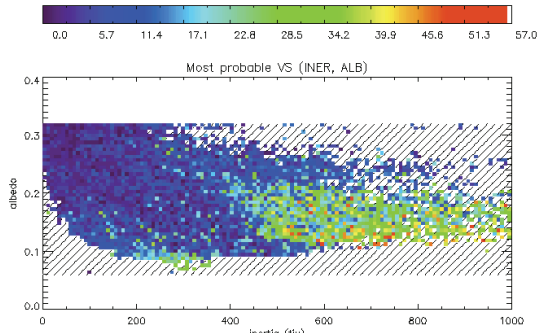
Figure 6: Most probable values of the rock abundance bin-distributions
