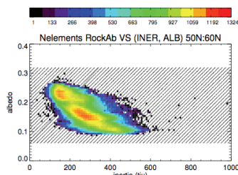
Figure 7: Density of points throughout the [I_k, \alpha_i] bins in the north band [50^{\circ}\text{N}:60^{\circ}\text{N}] .
