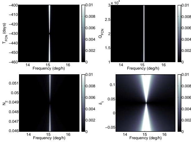
Fig. 1. Sensitivity of the gravimetric transfer function T^{(g)} to the parameters T_{FCN} , Q_{FCN} , N_2 , and \bar{\delta}_1 .
