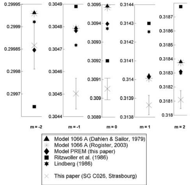
Figure 3. Comparison of the observed singlets of {}_0S_2 and their error bars from the SG C026 gravimeter at Strasbourg with the values observed by Ritzwoller et al. [1986], by Lindberg [1986] and with the predicted values for Earth models 1066A and PREM from various authors.
