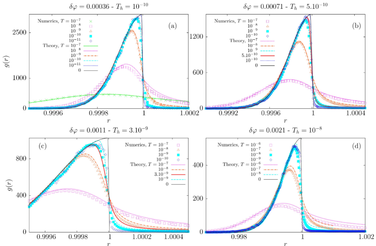
FIG. 15: (Color online) Pair correlations g_{glass}(r) above jamming predicted by theory (full lines) and measured in numerical simulations (symbols). The agreement is very good for T > T_h(\delta\varphi) , the values of T_h(\delta\varphi) are reported above the figures. Below T_h(\varphi) , the numerical curves do not evolve anymore, while the theoretical curves continue to evolve towards the T = 0 theoretical limit.
