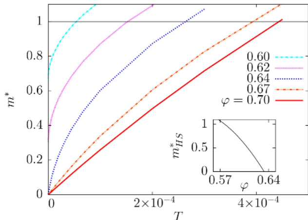
FIG. 7: (Color online) Optimal number of replicas m^* as a function of T , for several volume fractions. The inset shows the T \rightarrow 0 limit of m^* as a function of the volume fraction.
