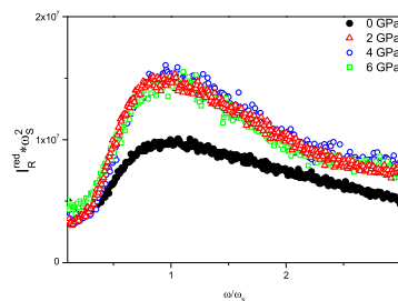
Figure 3. Reduced Raman intensity rescaled according to the scaling parameter \omega_s , at the indicated sample densities.
