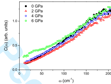
Figure 2. The Raman coupling function C(\omega) , calculated as the ratio between Raman and Neutron intensities at the same densities of figure 1.
