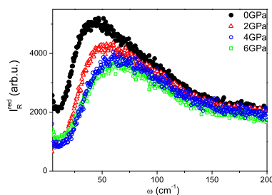
Figure 1. Room temperature low frequency HV reduced Raman intensity at different densities as indicated in the legend. The peak intensity reduces as the density is increased.
