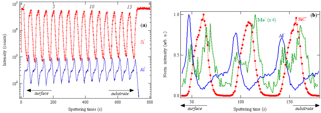
Figure 3: (a) Al - and Si - ion depth distribution of the Al/Mo/SiC multilayer; (b) SiC - , Al - and Mo - ion depth distributions of the 2 nd , 3 rd and 4 th periods of Al/Mo/SiC. For the sake of comparison, the Mo - profile intensity has been multiplied by a factor 4.
