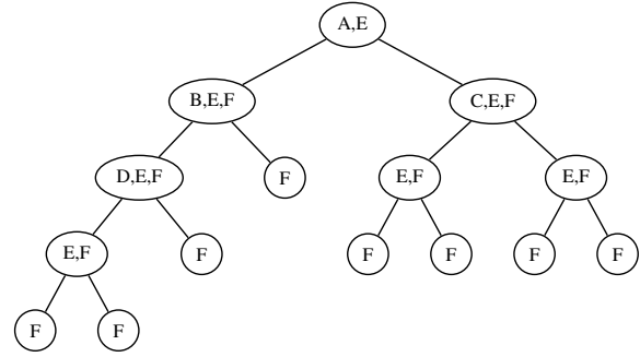
Figure 8: Another assignment of factors that is more economical than previous assignments in terms of regulator expressions.
