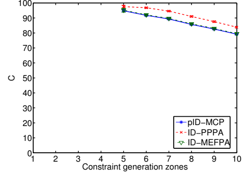
Fig. 5. The cost C according to the constraint generation zones in the LatticeSL(25,3) topology
