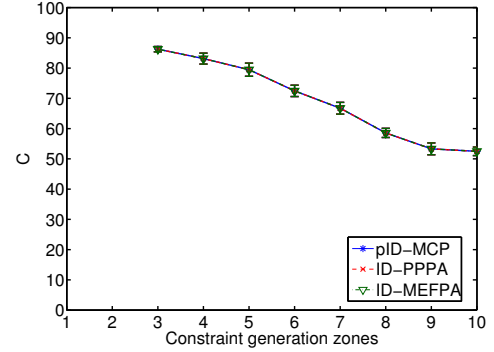
Fig. 6. The cost C according to the constraint generation zones in the LatticeFM(25,3) topology
