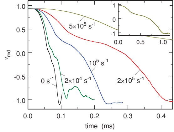
FIG. 10. (Color online) Simulation of the opening of the trap door. The plot shows the time evolution of the reduced volume v_{\text{red}} of the door when it is submitted to a pressure difference slightly larger than the critical pressure for buckling ( \Delta p \approx 15.6 kPa). The origin of times, t = 0 , is somewhat arbitrary. Langevin equations (3.15) were integrated numerically with a time step \Delta t = 0.2 ns. As indicated in the plots, the various curves were obtained with five different values of \gamma ranging from 0 to 5 \times 10^5 \text{ s}^{-1} . For \gamma = 5 \times 10^5 \text{ s}^{-1} , complete inversion ( v_{\text{red}} \approx -1 ) is achieved in about 1 ms, as shown in the small insert.
