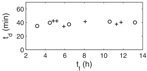
Figure 8. Measured deflation time t_d for 12 different firings of trap B versus the corresponding firing time interval t_f . Two series of 5 and 7 firings are shown (first series in circles, second series in crosses), and are separated by five days. Uncertainties on t_f are negligible compared to those on t_d ( \Delta t_d \sim 3 min). doi:10.1371/journal.pone.0020205.g008
