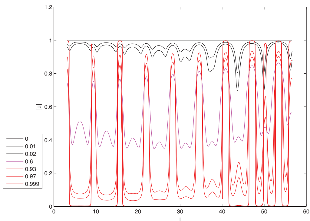
Figure 7. L^1 -minimization in two-body control, norm of the controls. The norm of the three-dimensional control versus longitude (the final longitude is fixed whereas the final time is free) is displayed for \lambda close to 0, \lambda = 0.6 , and \lambda close to 1. For \lambda = 0 , the minimum time problem is solved and |u| = 1 everywhere [16]. Conversely, for \lambda close to 1, the switching structure has been captured and almost-switches between 0 and 1 are observed on the norm.
