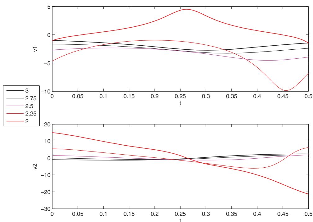
Figure 3. Energy minimization in quantum control, controls. The two components of optimal controls for \Gamma = 3, 2.75, 2.5, 2.25 and 2 are portrayed, illustrating the change of strategy when the physical parameter \gamma is decreased.
