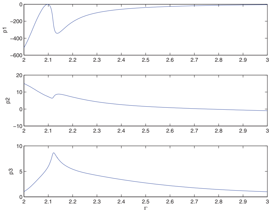
Figure 2. Energy minimization in quantum control, path of zeros. The initial adjoint state p_0 \in (\mathbf{R}^3)^* solution of the shooting function is computed when the homotopy parameter \Gamma decreases from 3 to 2.
