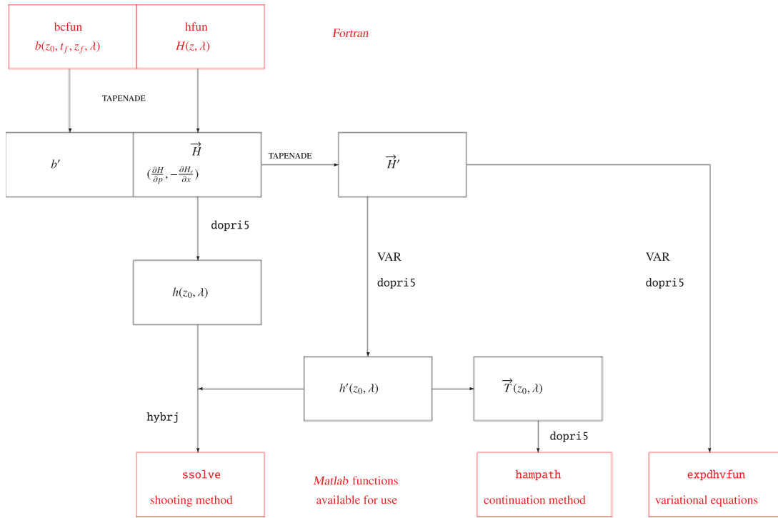
Figure 1. Overview of hampath.
