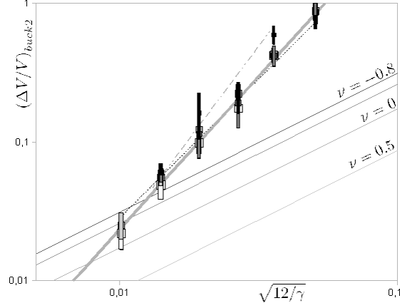
Figure 7: Points: relative volume variation at which the axisymmetric depression becomes “polygonal”, versus \sqrt{12/\gamma} (which is to be identified with d/R when \nu = 0 ). White: \nu = 0.5 ; light grey: \nu = 0 ; dark grey: \nu = -0.5 ; black: \nu = -0.8 . Wide grey line: equation 11. Continuous lines indicate the location of the first-order buckling for different Poisson’s ratio (from equation 8), under which only the spherical conformation is to be found. Non-continuous lines: in their domain of validity, equations describing the axisymmetric/wrinkled bowl transition published in previous works for \nu = 1/3 (see text): dotted black refers to [21], interrupted grey to [18].
