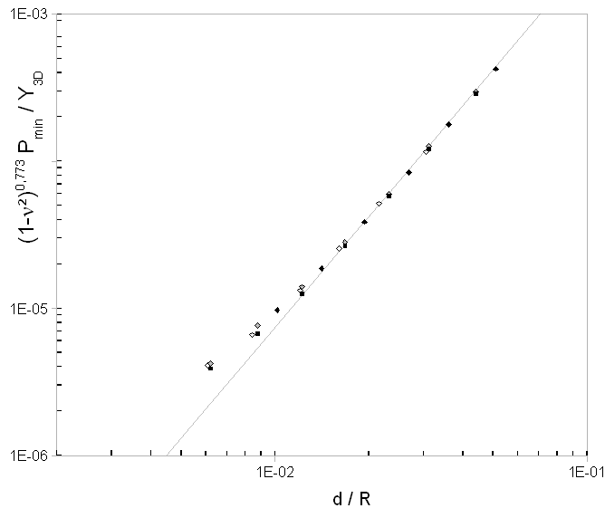
Figure 11: Pressure master curve after first buckling: \frac{\Delta P_{min}}{Y_{3D}} \times (1 - \nu^2)^{0.773} versus \frac{d}{R} . Black squares: \nu = 0.5 ; black diamonds: \nu = 0 ; light grey diamonds: \nu = -0.5 ; white diamonds: \nu = -0.8 . Continuous line: \frac{\Delta P_{min}}{Y_{3D}} \times (1 - \nu^2)^{0.773} = 0.75 \times \left(\frac{d}{R}\right)^{2.5} .
