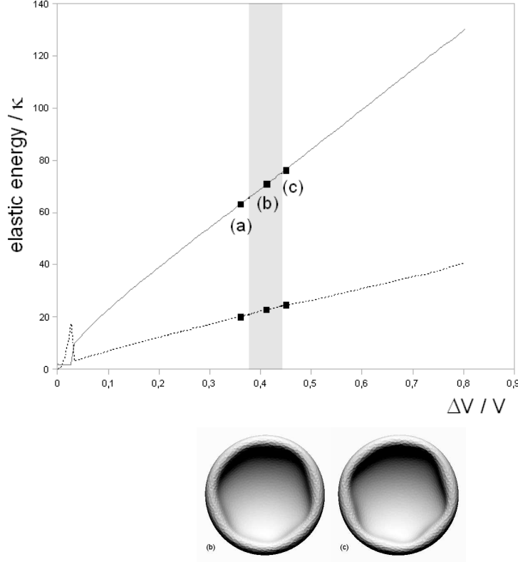
Figure 5: Deformation energies at different relative volume variations (volume step \approx 0.6\% of the initial volume), adimensionalized by the curvature constant \kappa , for \gamma = 9.33 \times 10^3 and \nu = 0.5 ( \frac{d}{R} = 0.031 ). Interrupted line: Hookean in-plane deformation energy, linked to the second significant term of eq. (6), i.e. \frac{1}{2}\epsilon_{ij}K_{ijkl}\epsilon_{kl} . Grey continuous line: elastic energy linked to the first significant term : \frac{1}{2}\kappa(c - c_0^*)^2 . This term does not vanish at \frac{\Delta V}{V} = 0 because c_0^* \neq c_0 ; in the total elastic energy, it is counterbalanced by the cst and the effective surface term expressed by \gamma_{eff} in equation (6). Effective surface energy (not represented here) varies at maximum by -0.33\kappa , and on an amplitude 0.03\kappa in the nonspherical conformations. Grey zone indicates the second transition from axisymmetric bowl shape to depression with inner wrinkles (“polygonal indentation”[18]), determined as explained in the text. First transition from sphere to axisymmetric bowl occurs through abrupt decrease of the in-plane deformation energy, at \frac{\Delta V}{V} = 0.03 .
