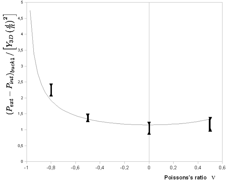
Figure 2: Pressure (\Delta P)_{buck1} = (P_{ext} - P_{int})_{buck1} at first sphere→bowl buckling, adimensionized by \Delta P_{Landau} . Error bars represent the range of this quantity for \gamma between 4.67 \times 10^3 and 2.33 \times 10^5 . Line: theoretical value 2 [3(1 - \nu^2)]^{-1/2} , from equation 7.
