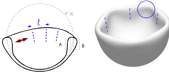
Figure 4: Left: schematisation of a spherical surface near complete deflation. Inner part of the rim endures a compressive stress in the direction indicated by the red double arrow. Relaxation of in-plane deformation occurs, for the thinnest shells, via undulation deformation, generating wrinkles (folds) all along the rim (examples schematized with blue interrupted lines). Length \ell stands for lateral extension of the wrinkles. Right: simulation with \gamma = 9.33 \times 10^3 , \nu = 0.5 ( \frac{d}{R} = 0.031 ) and \frac{\Delta V}{V} = 0.562 . Maxima of undulation are stressed with blue interrupted lines ; circle locates the zone of high curvature that forms the apex of the s-cone.
