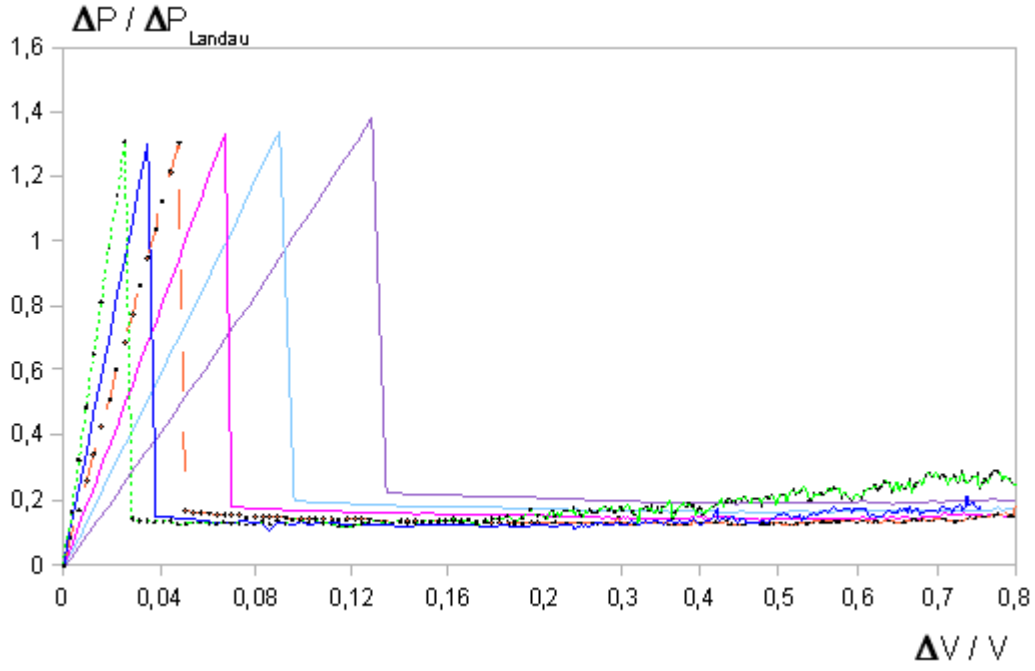
Figure 1: Pressure difference \Delta P = P_{ext} - P_{int} adimensionalized by \Delta P_{Landau} = Y_{3D} \left(\frac{d}{R}\right)^2 (or [12 Y_{2D} \kappa (1 - \nu^2)]^{1/2} / R^2 in 2D parameters), as a function of the relative volume variation, for surfaces of similar Poisson's ratio \nu = -0.5 . Dotted green: \gamma = 1.17 \times 10^5 ( \frac{d}{R} = 8.8 \times 10^{-3} ); blue: \gamma = 6.07 \times 10^4 ( \frac{d}{R} = 1.22 \times 10^{-2} ), interrupted orange: \gamma = 3.22 \times 10^4 ( \frac{d}{R} = 1.67 \times 10^{-2} ), magenta: \gamma = 1.17 \times 10^4 ( \frac{d}{R} = 2.31 \times 10^{-2} ), light blue: \gamma = 9.33 \times 10^3 ( \frac{d}{R} = 3.11 \times 10^{-2} ), parma: \gamma = 4.67 \times 10^3 ( \frac{d}{R} = 4.39 \times 10^{-2} ). Notice scale switch at \frac{\Delta V}{V} = 0.2 . Points (corresponding each to a minimization) emphasizes two curves with typical behaviour after buckling: increasing (green curve), and plateauing (orange) .
