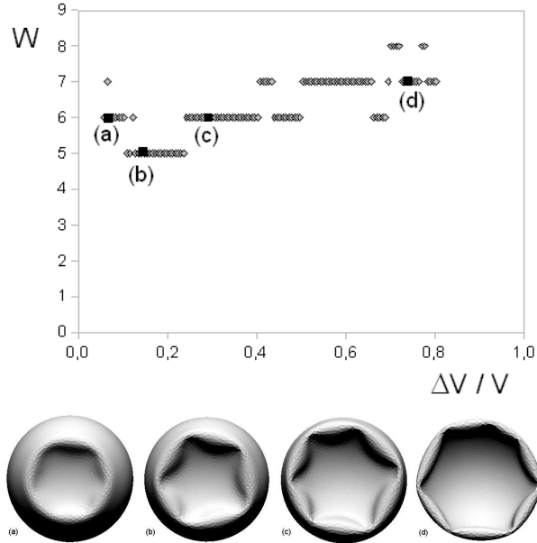
Figure 8: Number of wrinkles ( s -cones) held by the single depression after the secondary buckling of figure 5. Poisson’s ratio \nu = 0.5 ; Föppl-von Karman number \gamma = 6.06 \times 10^4 ( \frac{d}{R} = 0.0122 ). Lower part: conformations at points indicated on the main figure.
