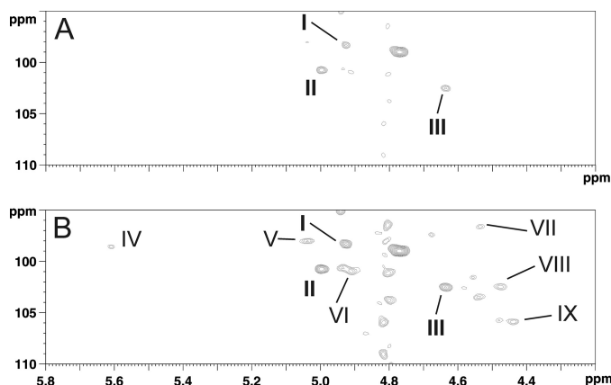
FIGURE 7. Detail of the anomeric region of ^{13}\text{C} , ^1\text{H} HSQC HR-MAS NMR analysis of bacterial cell surface of B. cereus from planktonic phase of growth. When looked at a low sensitivity, only signals from Ch HF-PS (I to III) can be seen (A), whereas increasing sensitivity permits to recover signals from Ne HF-PS (IV to IX) (B).
