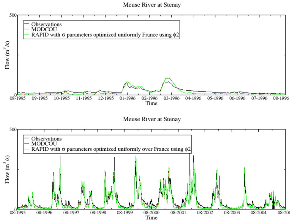
Figure 10 Comparison of 1995-1996 and 1995-2005 hydrographs for the Meuse River at Stenay obtained by MODCOU and RAPID with \sigma parameters optimized uniformly over France using the new cost function \phi_2
