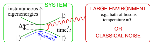
FIG. 1 (color online). We ask how coupling to an environment (with a given spectrum) affects the coherent oscillations of a system swept through a Landau-Zener transition.
