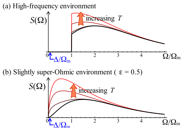
FIG. 3 (color online). Plots of S(\Omega) showing how weight below k_B T grows significantly as one increases T , while that above only grows slightly; the curves are for k_B T / \Omega_m = 0, 1/3, 2/3, \text{ and } 1 . In (a), there is no weight at low \Omega , so increasing T enhances \gamma via the level repulsion discussed in the text. For (b), there is enough weight at low \Omega that increasing T reduces \gamma .
