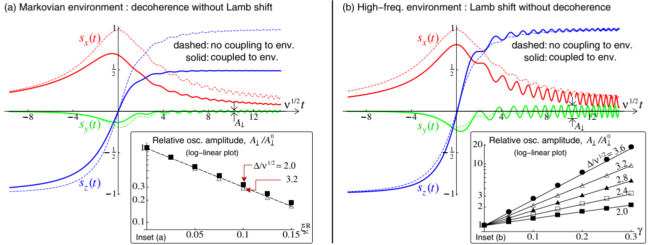
FIG. 2 (color online). The three spin components of the system swept through a Landau-Zener transition, given by numerical evolution of Eq. (3). The main plots in (a) and (b) have \Delta/\nu^{1/2} = 2.4 in the presence (solid curves) and absence (dashed curves) of environments. In (a), the environment induces decoherence, reducing the magnitude of the coherent oscillations, while, in (b), the environment induces a Lamb shift, which enhances such oscillations. In (a), the only nonzero \xi is \xi_z^R = 0.1 . The oscillation magnitude A_{\perp} is found by fitting s_y(t) for \nu^{1/2}t from 9.5 to 10.5. The inset shows its exponential decay with coupling strength, \xi_{sc}^R , at a rate which appears to be \Delta -independent. In (b), the only nonzero \xi is \xi_y^R = -\gamma\Delta , with \gamma = 0.3 , for which Eq. (3) reduces to Eq. (5). The inset shows A_{\perp} growing exponentially with environment coupling; the solid lines are the hypothesis that A_{\perp} = (1 - \gamma)^{1/2}A_{\perp}^0[\Delta(1 - \gamma)^{1/2}] , where A_{\perp}^0[x] is given by Eq. (2). Analysis of oscillations of s_x(t) gives identical results.
