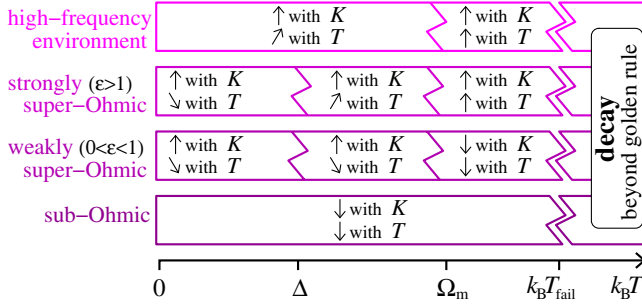
FIG. 4 (color online). Regimes of behavior of the coherent-oscillation magnitude, A_{\perp} . Exponentially strong enhancement with increasing coupling is indicated by “ \uparrow with K ” (and exponential reduction by “ \downarrow with K ”). Exponentially strong increases and decreases with increasing temperature are indicated by “ \uparrow with T ” and “ \downarrow with T ,” while weaker temperature dependences are indicated by “ \nearrow with T ” and “ \searrow with T .”
