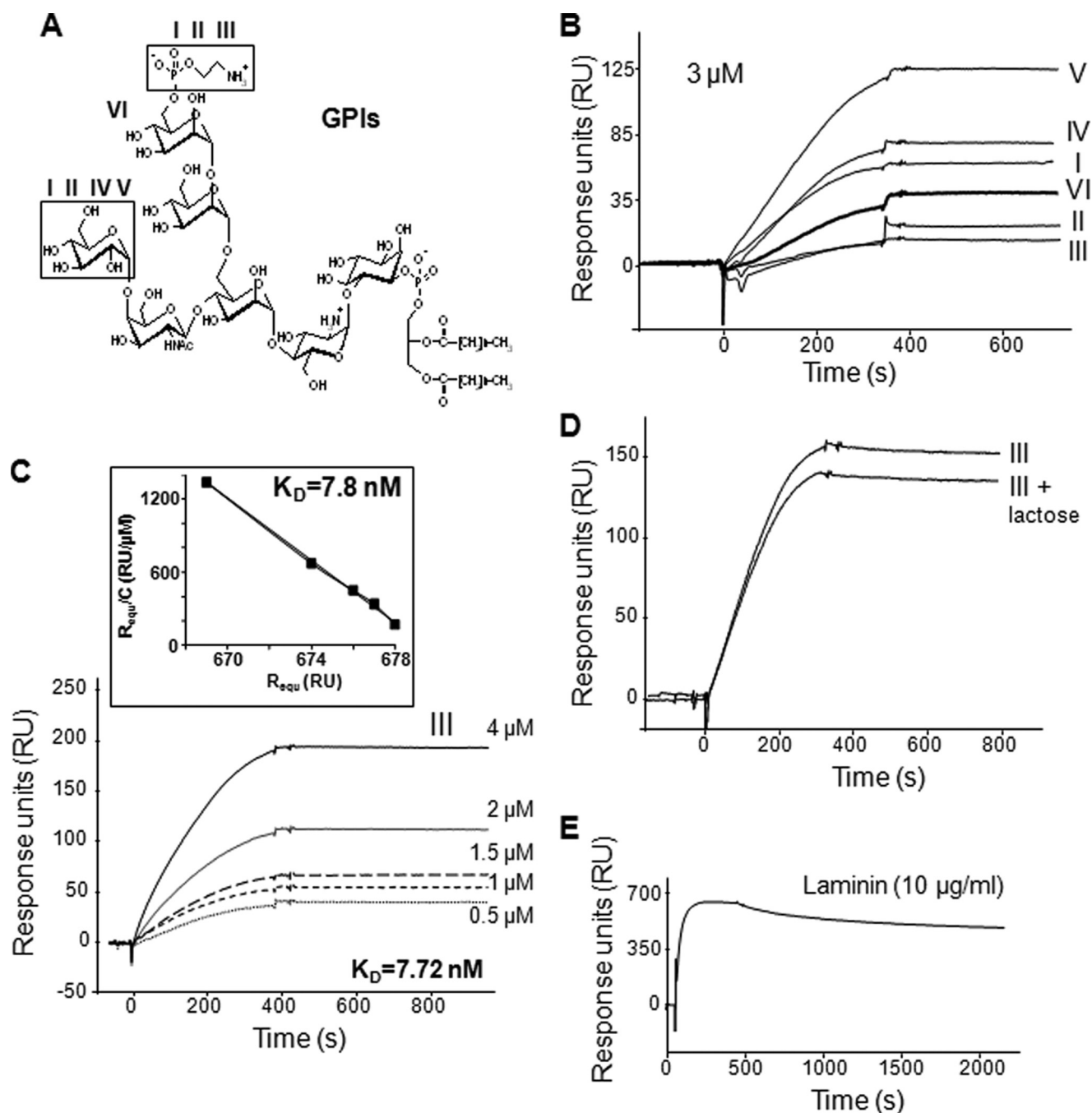
FIGURE 1. GPIs of T. gondii associate with galectin-3. A, structures of T. gondii GPIs: GPIs I and II, (EtN-P)-Man \alpha 1-2Man \alpha 1-6(Glc \alpha 1-4GalNAc \beta 1-4)Man \alpha 1-4GlcNAc-Ino-P-DAG; GPI III, (EtN-P)-Man \alpha 1-2Man \alpha 1-6(GalNAc \beta 1-4)Man \alpha 1-4GlcNAc-Ino-P-DAG; GPIs IV and V, Man \alpha 1-2Man \alpha 1-6(Glc \alpha 1-4GalNAc \beta 1-4)Man \alpha 1-4GlcNAc-Ino-P-DAG; and GPI VI, Man \alpha 1-2Man \alpha 1-6(GalNAc \beta 1-4)Man \alpha 1-4GlcNAc-Ino-P-DAG. GPIs I and II, and GPIs IV and V differ in their diacylglycerol composition with palmitic and stearic acids as predominant fatty acids. EtN, ethanolamine; P, phosphate; Man, mannose; Glc, glucose; GalNAc, acetylgalactosamine; GlcN, glucosamine; Ino, inositol; DAG, diacylglycerol. B-E, SPR analysis of the interaction of immobilized galectin-3 with the six different T. gondii GPIs (I-VI) at 3 \mu\text{M} (B); different concentrations of T. gondii GPI III with Scatchard plot analysis of the sensorgram data shown in the inset (slope = -127.4) (C); GPI III at 3 \mu\text{M} in the presence of 30 mM lactose (D); or laminin at 10 \mu\text{g/ml} (E). Results are expressed as RU (proportional to the quantity of molecules) after the subtraction of the nonspecific binding. Sensorgrams are representative of independent experiments with similar results.
