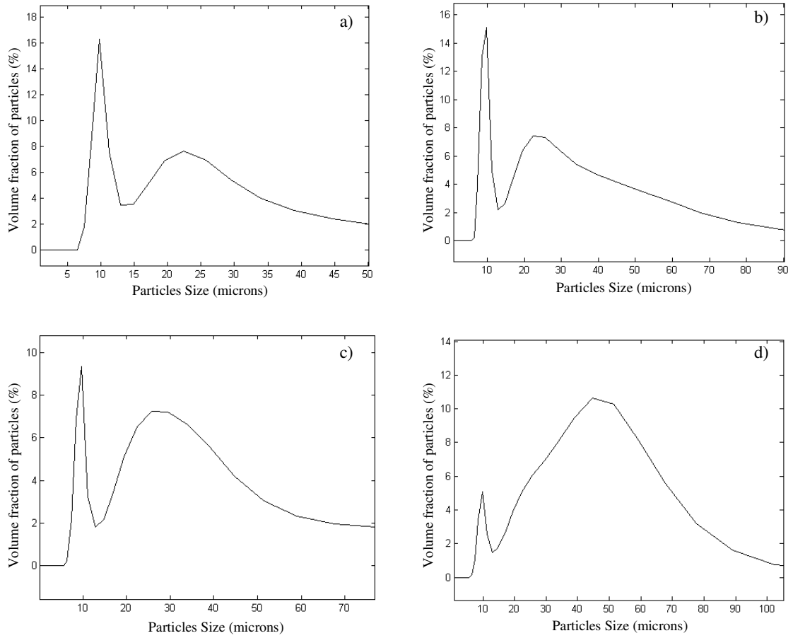
Figure 5. Particles size distribution (in volume) of sieved powder with a theoretical diameter: a) lower than 20 \mu\text{m} , b) in the range 20-30 \mu\text{m} , c) in the range 30-40 \mu\text{m} , d) in the range 40-50 \mu\text{m} .
