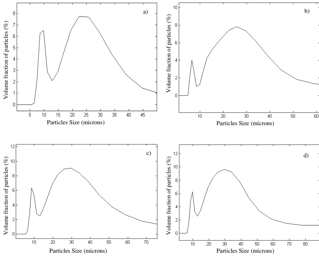
Figure 11. Particles size distribution before (a and c) and after (b and d) the oxidation treatment of sieved powder in the range 20-30 \mu\text{m} (a and b) and 30-40 \mu\text{m} (c and d).
