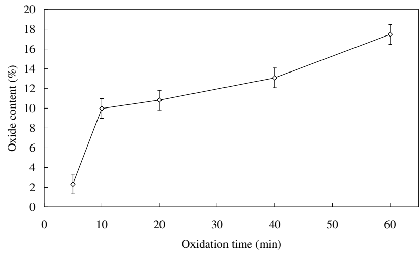
Figure 8. Effect of the time of treatment on the oxide content ( 1.5 \text{ A.dm}^{-2} , 20 %, 30-40 \mu\text{m} ).
