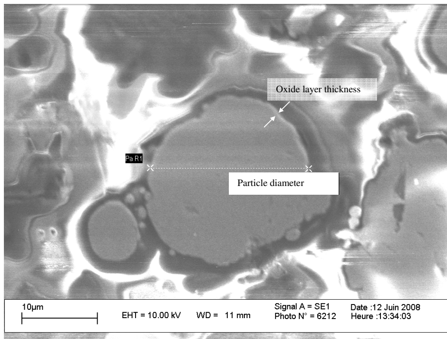
Figure 12. SEM visualisation of Al micrometric particle with oxide layer.
