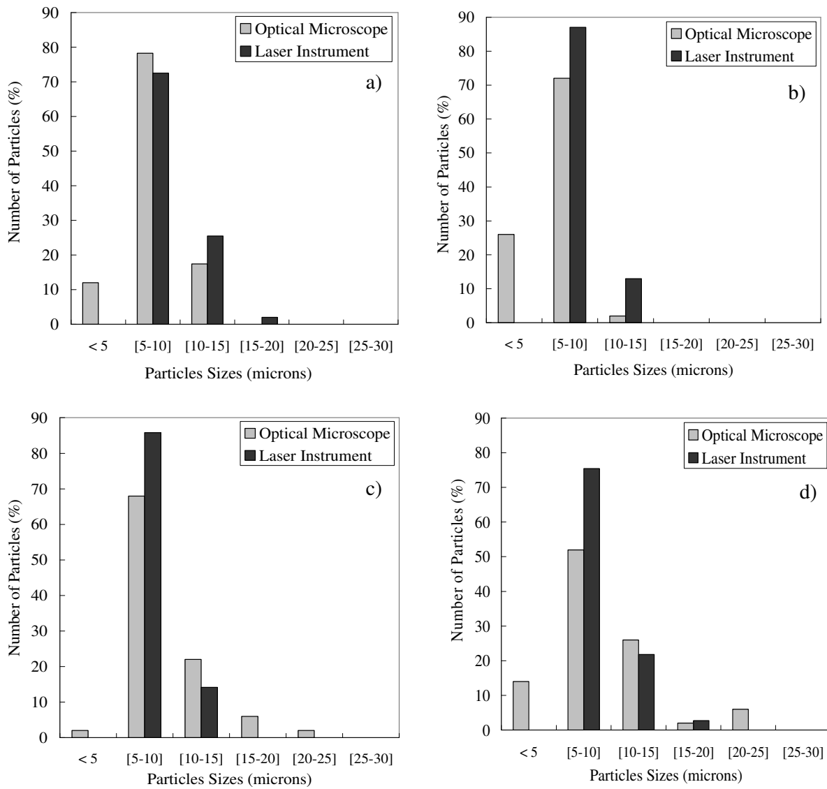
Figure 4. Particles size distribution (in number) of sieved Al powder with a theoretical diameter: a) lower than 20 \mu\text{m} , b) in the range 20-30 \mu\text{m} , c) in the range 30-40 \mu\text{m} , d) in the range 40-50 \mu\text{m} .
