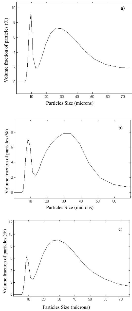
Figure 6. Particles size distribution (in volume) of sieved powder in the range 30-40 \mu\text{m} after one sieving (a), two sieving (b) and three sieving (c).
