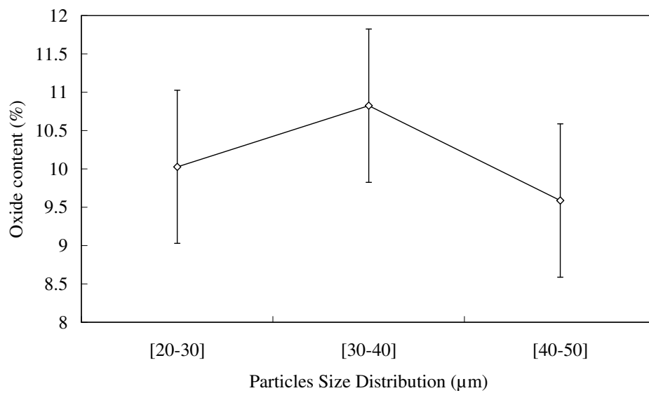
Figure 10. Oxide content of sieved powder treated with the same test parameters (20 min, 1.5 \text{ A.dm}^{-2} , 20 %) – TGA measures.
