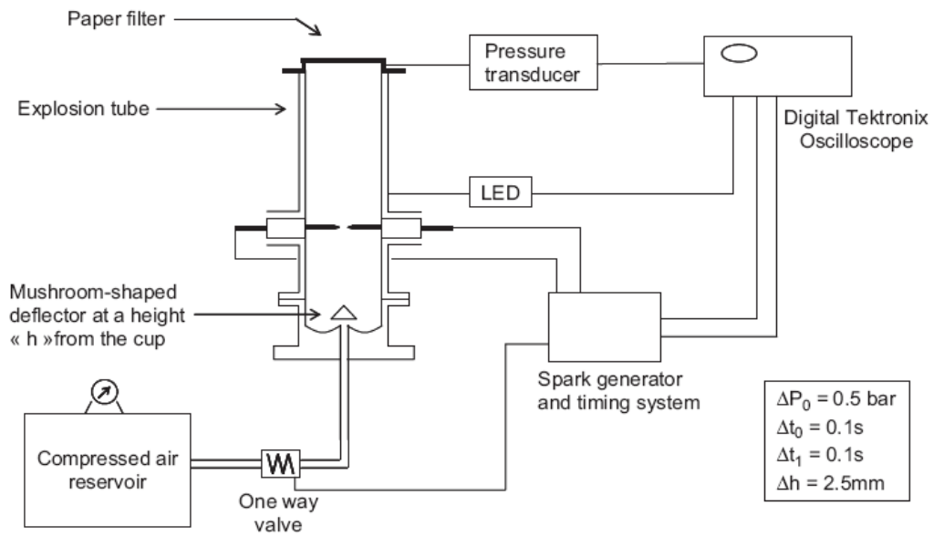
Figure 2. Experimental bench with Hartmann tube used by Baudry et al. to test the explosibility of Al powder [16].
