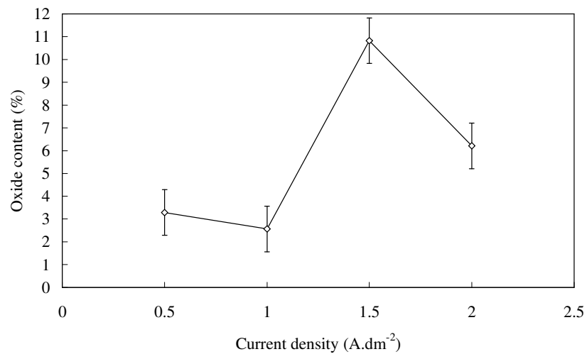
Figure 9. Effect of the current density on the oxide content (20 min, 20 %, 30-40 \mu\text{m} ).
