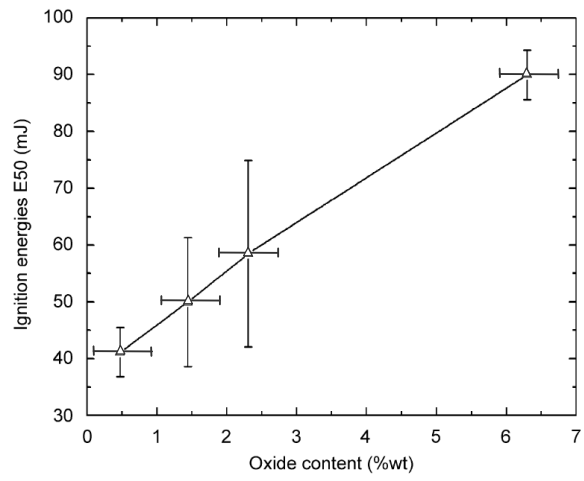
Figure 1. Mitigation effect of the oxide content in the Al powder on the ignition energy [16].
