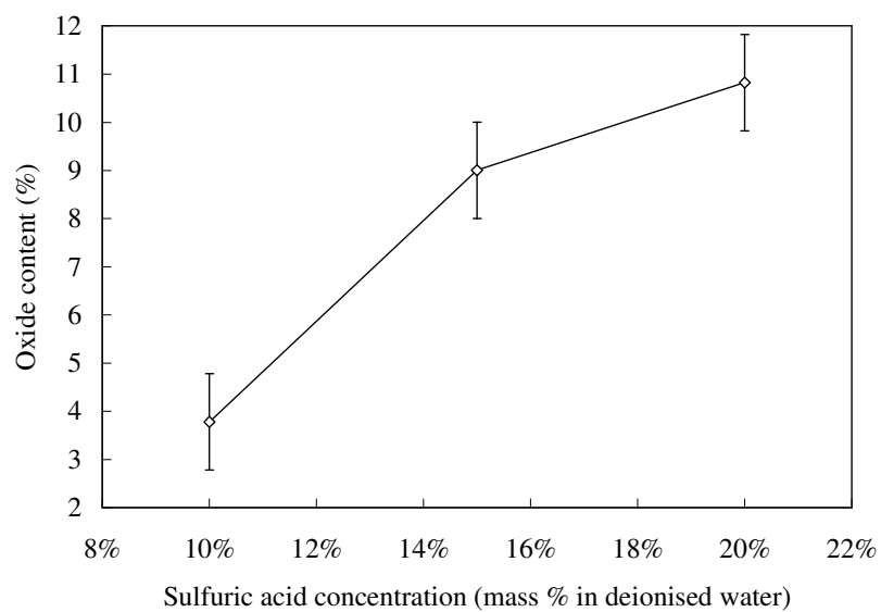
Figure 7. Effect of the acid concentration on the oxide content (20 min, 1.5 \text{ A.dm}^{-2} , 30\text{-}40 \text{ }\mu\text{m} ).
