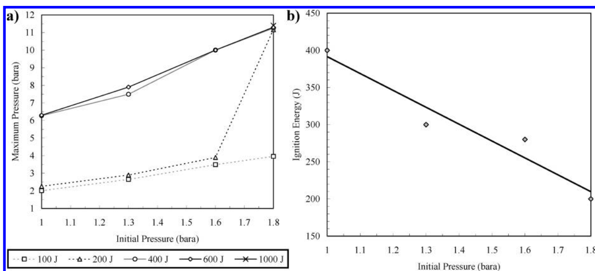
Figure 8. (a) Maximum pressure after explosion depending on initial pressure for several ignition energies (equivalence ratio of 0.3, volume of 1\text{ m}^3 ); (b) initial pressure dependence of the ignition energy (volume of 1\text{ m}^3 , equivalence ratio of 0.3).
