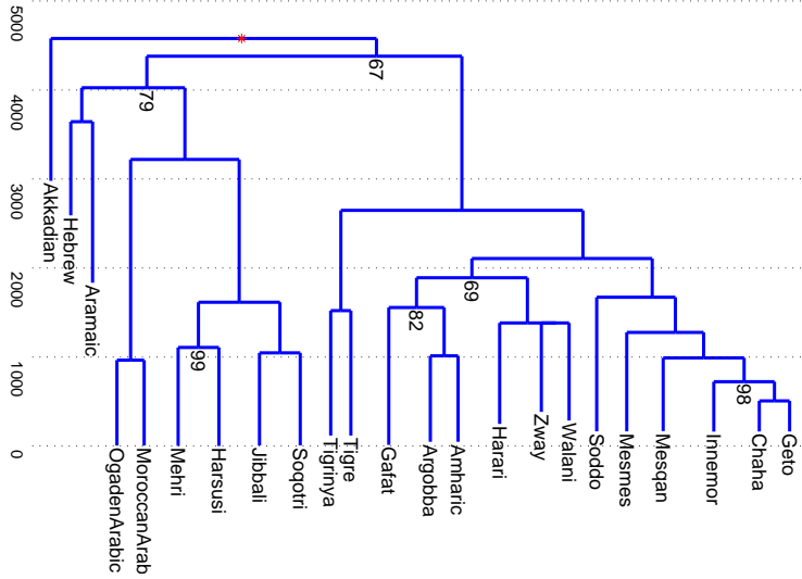
FIGURE 2. Consensus tree for the KEAM-23 data. Edge lengths are proportional to posterior mean time to branching. Edges thresholded at support 50% posterior probability. Numbers on nodes give posterior probability for the edges above. Unnumbered edges have posterior support equal one.
