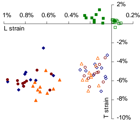
Fig. 1: Longitudinal (L) versus tangential (T) strains measured on normal wood (open symbols) and tension wood (filled symbols). Square = HT strain on set B ( \varepsilon_{HT}^{\text{B}} ); triangle = pure drying strain ( \varepsilon_{PD}^{\text{B}} ) on set B; circle = total strain on set B ( \varepsilon_{tot}^{\text{B}} ); diamond = total strain ( \varepsilon_{tot}^{\text{A}} ) on set A.
