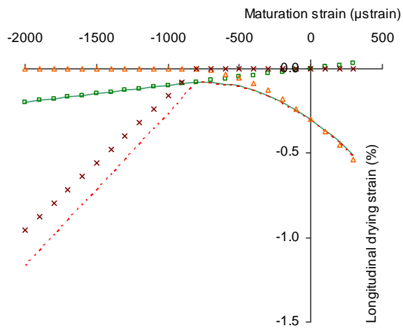
Fig. 3: Schematic model of the 3 cumulative contributions to longitudinal shrinkage as a function of the maturation strain. Green squares: strain caused by stress release; orange triangles: strain caused by water departure; crosses: strain caused by G-layer collapse. Plain line (green): resulting shrinkage on wood from species not producing G-layer; dotted line (red): resulting shrinkage on wood from species producing G-layer.
