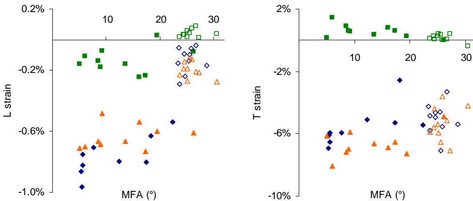
Fig. 2: Longitudinal (L) and tangential (T) strains measured on samples supposed to be normal wood (open symbols) and tension wood (filled symbols) as a function of their microfibril angle (MFA). Square = HT strain on set B ( \varepsilon_{\text{HT}}^{\text{B}} ); triangle = pure drying strain on set B ( \varepsilon_{\text{PD}}^{\text{B}} ); diamond = total strain on set A ( \varepsilon_{\text{tot}}^{\text{A}} ).
