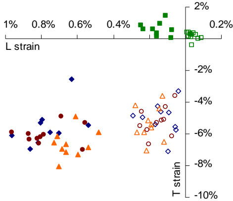
Fig. 1: Longitudinal (L) versus tangential (T) strains measured on normal wood (open symbols) and tension wood (filled symbols). Square = HT strain on set B ( \varepsilon_{\text{HT}}^{\text{B}} ); triangle = pure drying strain ( \varepsilon_{\text{PD}}^{\text{B}} ) on set B; circle = total strain on set B ( \varepsilon_{\text{tot}}^{\text{B}} ); diamond = total strain ( \varepsilon_{\text{tot}}^{\text{A}} ) on set A.
