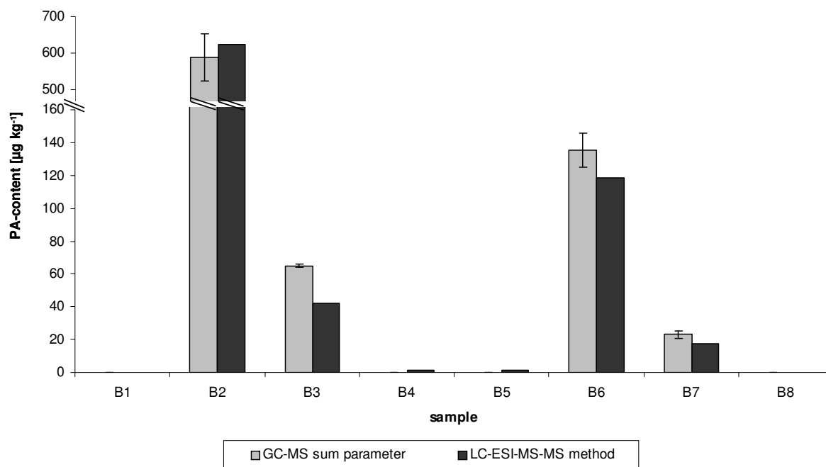
Figure 4: Comparison of the total PA-content of randomly picked raw honeys (n = 8; set B) calculated in retronecine equivalents. Left (gray) bars GC-MS sum parameter approach (SD; n = 3), right (black) bars LC-MS-MS method, respectively.
