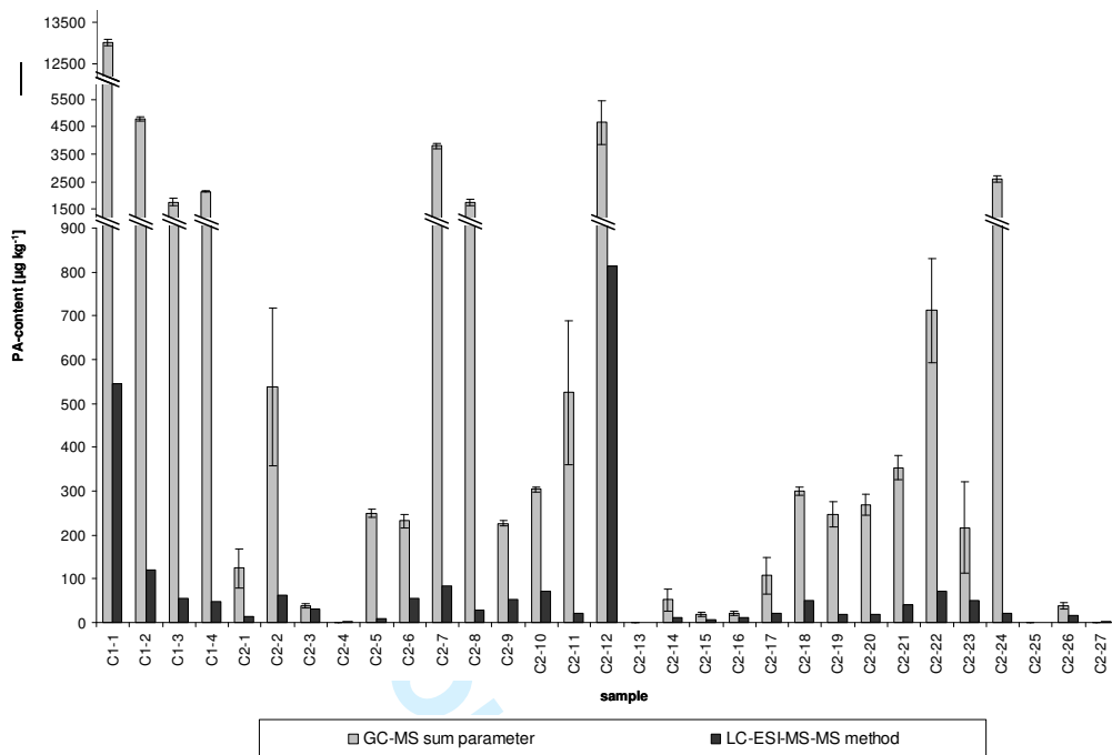
Figure 5: Comparison of the total PA-content of Jacobaea vulgaris honeys (n = 31; set C; Veluwe region; The Netherlands) calculated in retronecine equivalents. Left (gray) bars GC-MS sum parameter approach (SD; n = 3), right (black) bars LC-MS-MS method, respectively.
