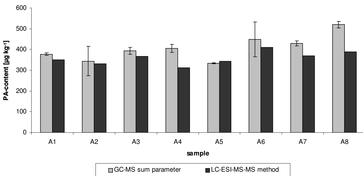
Figure 3: Comparison of the total PA-content of Echium honeys (n = 8; set A; New Zealand) calculated in retronecine equivalents. Left (gray) bars GC-MS sum parameter approach (SD; n = 3), right (black) bars LC-MS-MS method, respectively.
