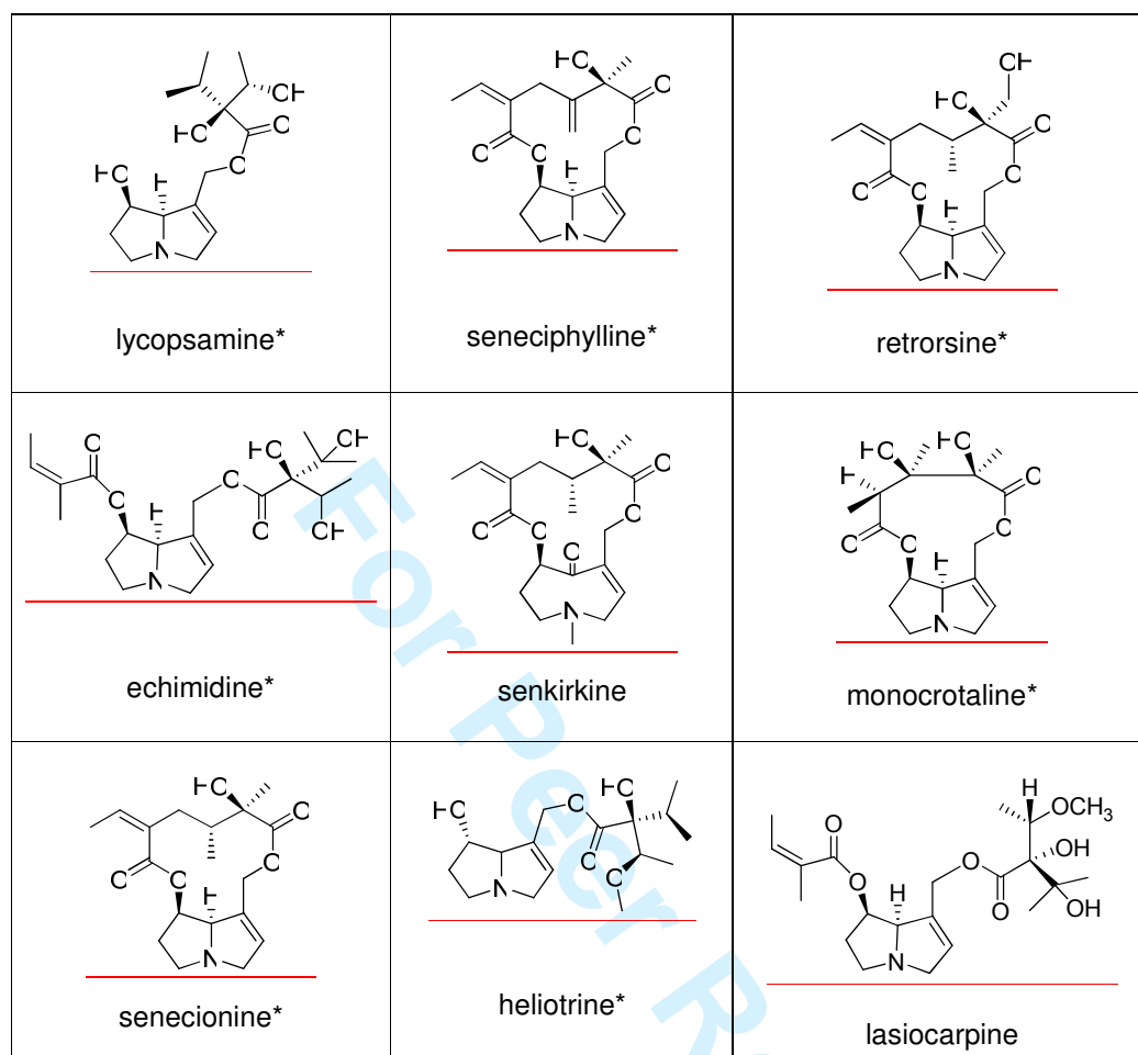
Figure 1: Structures of commercially available PAs used as reference compounds in this study. * The N -oxides of echimidine, heliotrine, lycopsamine, monocrotaline, retrorsine, senecionine and seneciphylline were chemically synthesized.
