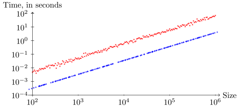
Figure 3: Time for generating an increasing binary tree of given size
