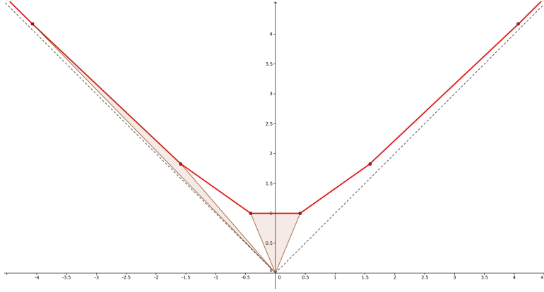
Figure 4: The two shaded regions have the same area. This area is the coarea of the polygon.
