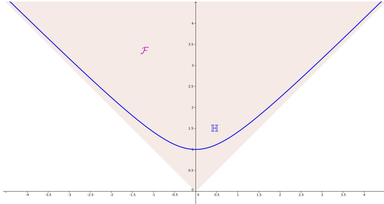
Figure 1: The cone \mathcal{F} of future time-like vectors and the curve \mathbb{H} of unit future time-like vectors.
