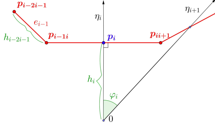
Figure 3: Notations for a t -convex polygon.
