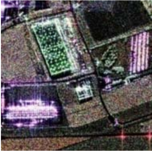
Figure 6. Pauli representation of the first dataset.
