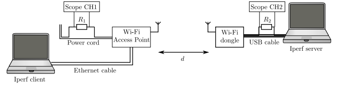
Fig. 3: Power measurement setup
