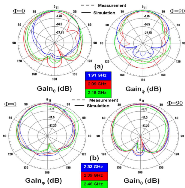
Figure 7. Radiation Patterns (a) Port 1 (b) Port 2
