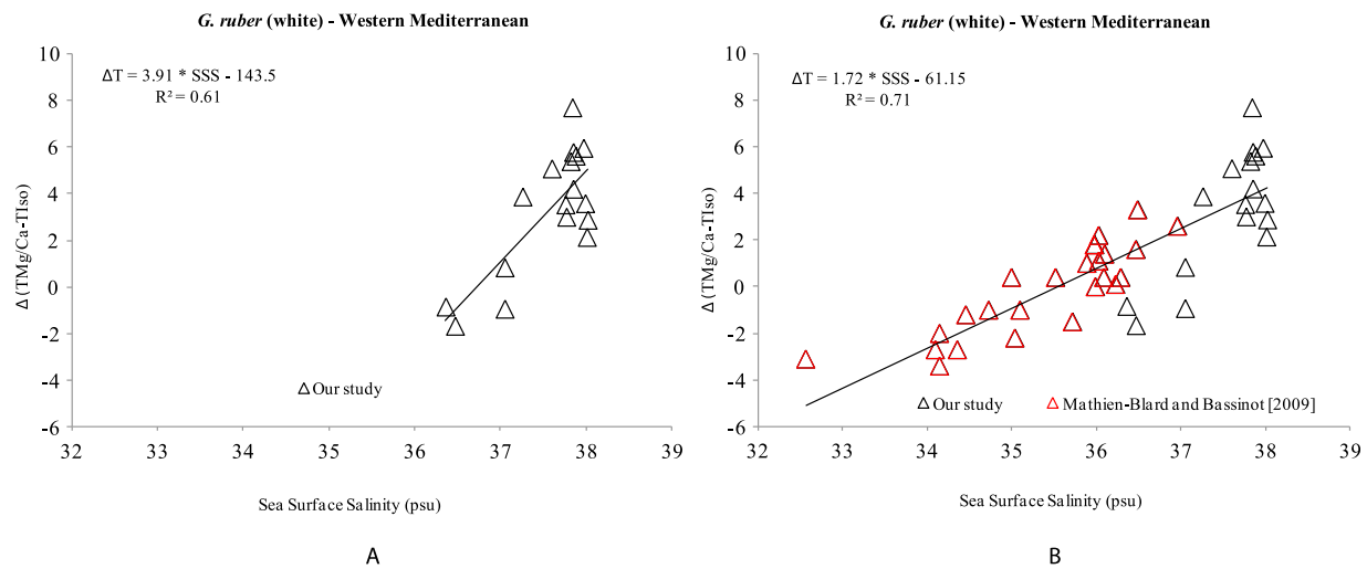
Figure 7. (a) Series of our Western Mediterranean \Delta T ( = T_{Mg/Ca} - T_{iso} ) plotted against atlas-derived sea surface salinities [ MEDAR Group , 2002] and [ Antonov et al. , 2006] for G. ruber (white). (b) Series of \Delta T ( = T_{Mg/Ca} - T_{iso} ) plotted against atlas-derived sea surface salinities [ MEDAR Group , 2002] and [ Antonov et al. , 2006] for G. ruber (white). Temperatures corresponding Mg/Ca ratios were calculated based on calibration from Anand et al. [2003] as explained in the text. \Delta T is the difference between T_{Mg/Ca} and T_{iso} calculated from \delta^{18}O_w -derived isotopic temperatures calculated using the equation of Shackleton [1974]. West Mediterranean core tops are symbolized by black triangles; Indo-Pacific and North Atlantic core tops analyzed by Mathien-Blard and Bassinot [2009] are shown as red triangles. The black line materializes the linear regression calculated taking into account all the data on the graphic and for both Figures 7a and 7b, it results highly significant ( *** = P \ll 0.001 ).
