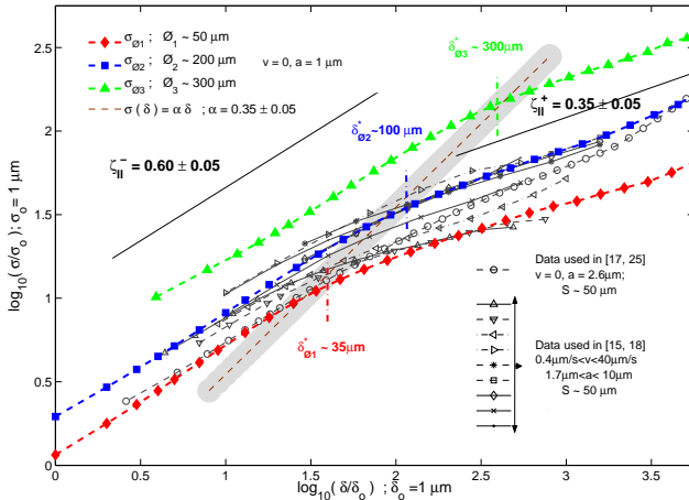
FIG. 4: Effect of disorder on the scaling of interfacial crack fronts. We plot the rms \sigma of the height fluctuations \Delta y as a function of the scale \delta for crack fronts at rest and samples blasted with glass beads of various diameters \varnothing_1 \sim 50 \mu\text{m} , \varnothing_2 \sim 200 \mu\text{m} and \varnothing_3 \sim 300 \mu\text{m} . The line \sigma(\delta) = 0.35 \delta separates the two scaling regimes. To insist on the robustness of our results, we add various data obtained during previous experiments with many different experimental conditions: glass-aluminium powder with a typical size around S \sim 50 \mu\text{m} and crack front propagating at various velocities v [16, 18, 19, 26].
