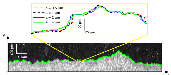
FIG. 1: A typical fracture (using glass beads of a diameter \varnothing_1 \sim 50\mu\text{m} for roughening the samples) and a zoom of the crack front y(x) to emphasize the effect of the optical resolution given by the pixel size a .
