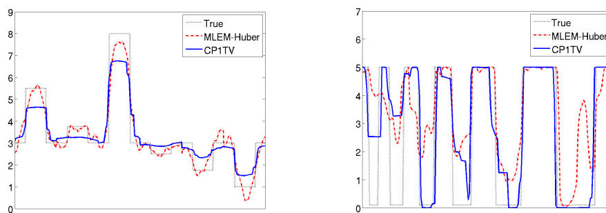
Figure 13: Profile of the PET contrast (left) and resolution (right) phantom reconstruction results for 60 angles of projections and a noise level of fcount = 2e5 .
