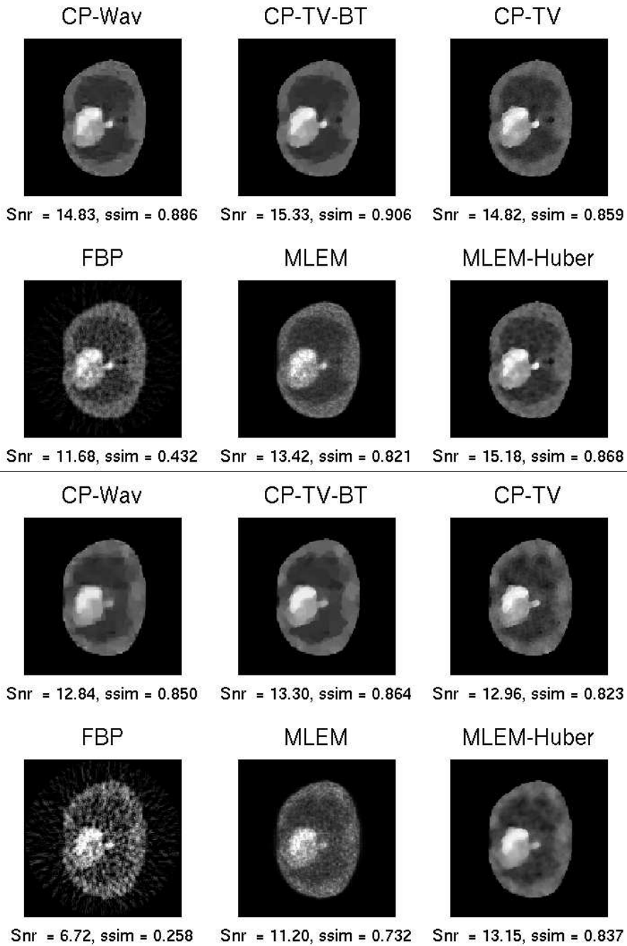
Figure 10: TEP reconstructions, top two rows: detector efficiency f_{count}=500000 , bottom two rows: detector efficiency f_{count}=100000 .
