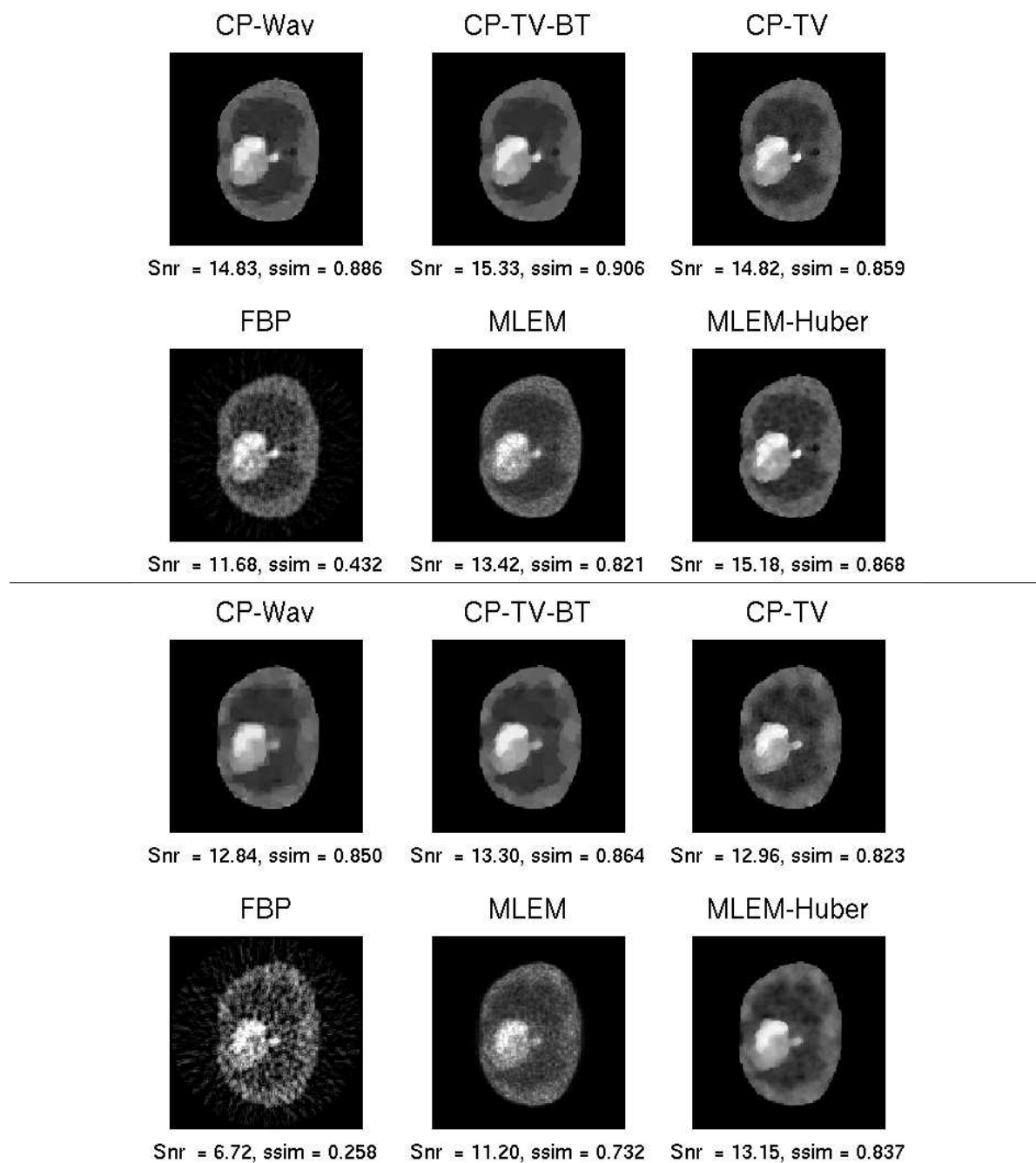
Figure 10: TEP reconstructions, top two rows: detector efficiency f_{count}=500000 , bottom two rows: detector efficiency f_{count}=100000 .
