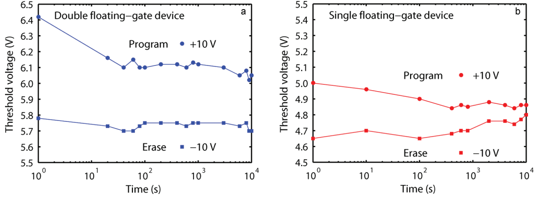
Figure 6. Retention properties of the devices with single Si floating gate and double floating gates (Si/Ge) at room temperature: (a) Memory window of the double floating-gate memory device with programming/erasing at \pm 10 V for 10 s. The threshold voltage was defined at I_d = 0.5 nA and V_d = 500 mV. After 100 s, the memory window width gets mostly saturated with time. (b) Memory window of the single floating-gate memory device with programming/erasing at \pm 10 V for 10 s. The memory window width tends to zero with increasing time.
