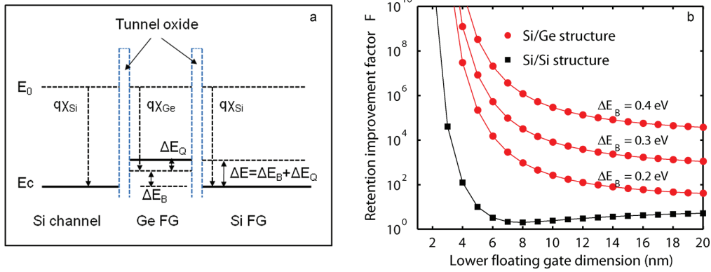
Figure 7. Energy-band diagram of the double floating-gate memory and the retention improvement factor for the double floating-gate devices with either two Si floating gates (Si/Si) or the combination of Si and Ge floating gates (Si/Ge). (a) Energy band diagram in a low or zero gate voltage configuration. The energy barrier \Delta E is the sum of the conduction-band offset \Delta E_B between Ge and Si and the characteristic energy \Delta E_Q induced by Coulomb blockade and quantum confinement effects. (b) Calculated retention improvement factors for two types of structures (Si/Si and Si/Ge) as a function of the lower floating gate dimension d .
