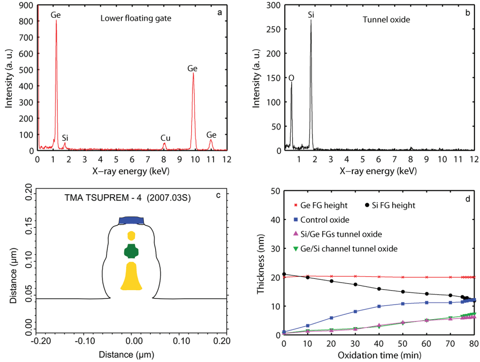
Figure 4. Energy dispersive X-ray spectroscopy (EDS) spectra and process simulation results: (a) EDS for the lower floating gate with an hexagonal shape, showing that it is made of pure Ge; (b) EDS for both tunnel oxides, indicating that it is a \text{SiO}_2 layer; (c) simulated device center based on TSUPREM-4; (d) five main geometrical parameter evolutions of the double floating gate memory device (two floating gate heights, two tunnel oxide thicknesses and control oxide thickness) as a function of oxidation time at 750 °C.
