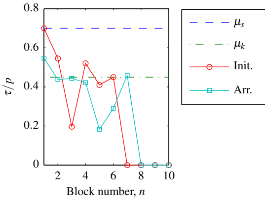
Fig. 3 Tangential force distribution at initiation of a microslip-event ( \circ ). Block 1 has reached its slip threshold ( \tau/p = \mu_s ). The event involves all blocks from 1 to 6 ( i.e. a precursor of length L_p/L = 0.6 ), leading to a modified tangential force distribution at arrest ( \square ). Results obtained using N = 10 (as in [17]) and \theta = 0 .
