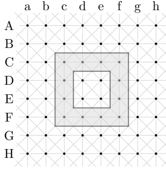
Figure 2: Notation for vertices in the neighbourhood of a frame.
