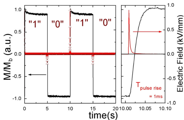
FIG. 5. (Color online) MOKE measurement of the magnetic element magnetization: a negative pulse voltage switches M in the “0” state and a positive pulse into the “1” state. Left: sequence over 20 s. Right: zoom around t = 10 s.
