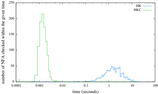
Figure 7. Distribution of the execution times of HK and HKC, for the 1000 NFA with 100 states and 2 letters used in Table I.
