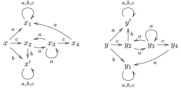
Figure 8. The relation built by HKC(x, y) is not included in HK(x, y) .
