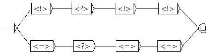
Figure 7.20: ELAG grammar without any constraint
