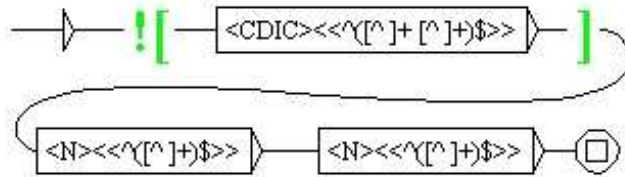
Figure 6.15: Advanced use of contexts
