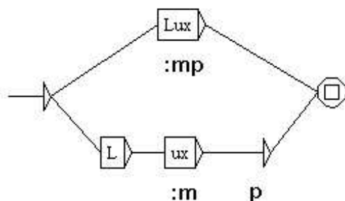
Figure 6.2: Two equivalent paths in an inflection grammar
