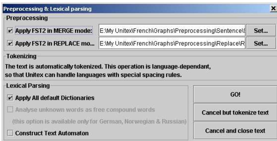
Figure 2.8: Preprocessing Window
